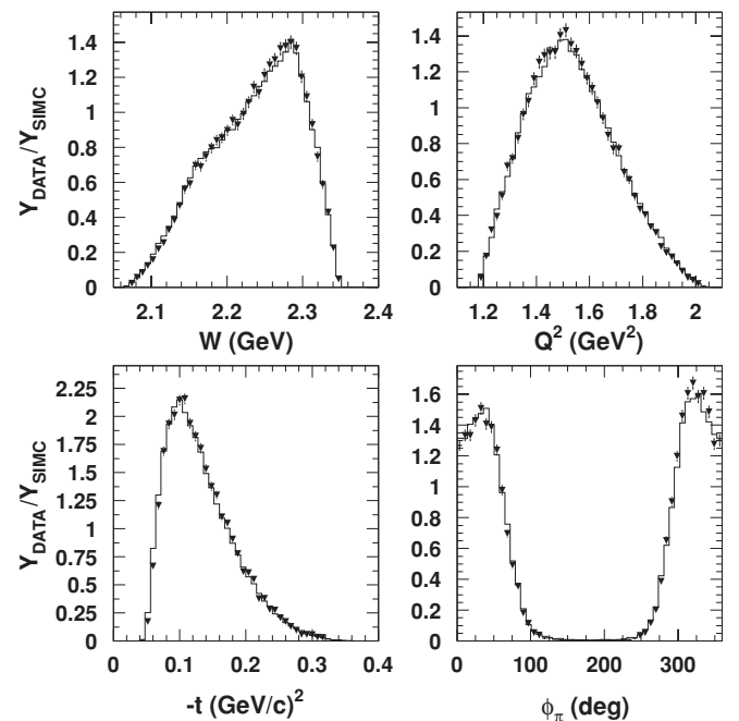
FIG. 13. Comparison of data (triangles) and SIMC (histogram) for the quantities W , Q^2 , -t , and \phi_\pi . The distributions were normalized to each other by one global scale factor.
