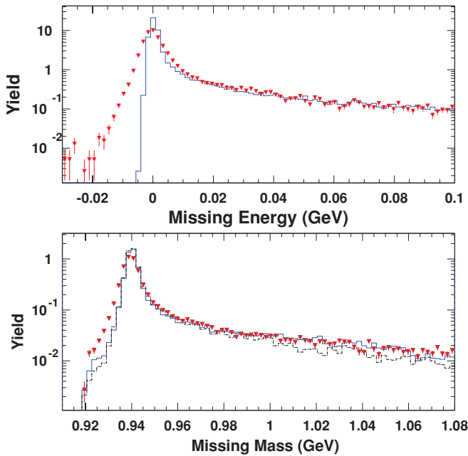
FIG. 14. (Color online) Comparison between data (triangles) and SIMC (histogram) for the missing-energy distribution for one of the {}^1\text{H}(e, e'p) kinematics (top) and for the missing-mass distribution for a representative {}^1\text{H}(e, e'\pi^+)n case (bottom). The solid histogram includes radiative effects and pions that pass through the HMS collimator. The latter events produce an additional contribution in the region M_m = 1.025\text{--}1.07 GeV. The dashed histogram represents simulated events without the effect of collimator punch-through.
