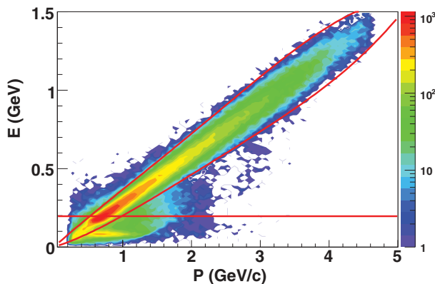
FIG. 2. (Color) Energy deposited by the electron candidates in the electromagnetic calorimeter vs momentum. The lines show the selection cuts for good electrons as described in the text.
