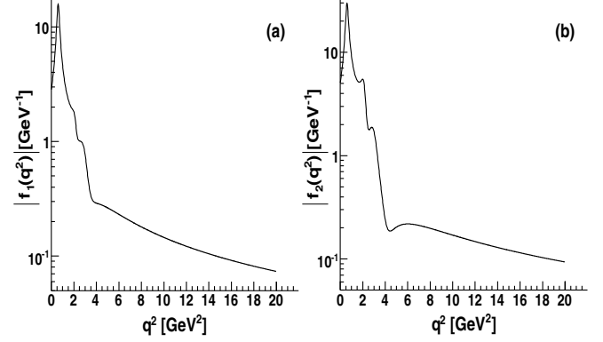
FIG. 2. q^2 dependence of the \gamma^*\pi a_1 transition form factors f_1, f_2 (41).
