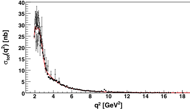
FIG. 1. (Color online) Total cross section data for the annihilation e^+e^- \rightarrow \pi^+\pi^-\pi^+\pi^- from [5,26–28]. The line represents the fit of the total cross section (16) for the reaction e^+ + e^- \rightarrow a_1 + \pi with VMD-based model of transition form factors (41).
