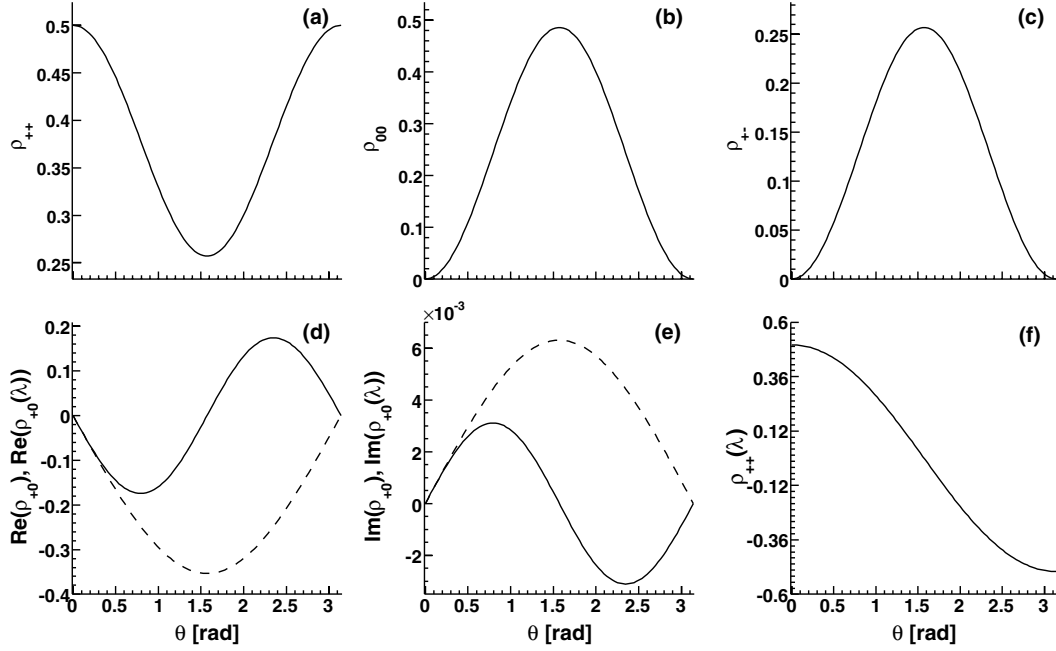
FIG. 5. Angular dependence of the elements of the spin density matrix \rho_{++} , \rho_{00} , \rho_{+-} , \rho_{+0} at q^2 = 2 \text{ GeV}^2 , in case of unpolarized collision (solid lines) from Eqs. (30), (31). In case of longitudinally polarized electrons the corresponding elements are shown also [dashed lines, (d),(e)] from Eqs. (37) and (f) from Eq. (36).
