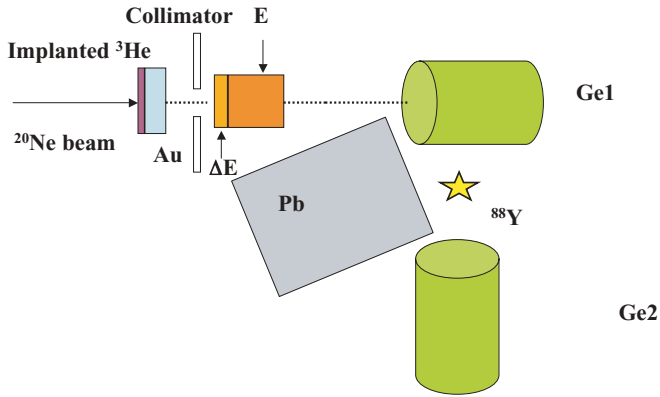
FIG. 1. (Color online) Experimental setup (not to scale). A layer of ^3\text{He} was implanted in a Au foil. \alpha particles from the ^3\text{He}(^{20}\text{Ne},\alpha)^{19}\text{Ne} reaction were detected in 25\ \mu\text{m} \Delta E and 500\ \mu\text{m} E detectors. The Ge detector aligned to the beam axis was used to detect ^{19}\text{Ne} \gamma rays. The second Ge detector viewed a weak ^{88}\text{Y} source shielded from the target by a Pb absorber.
