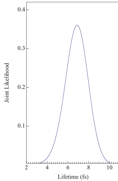
FIG. 8. (Color online) Joint likelihood for the lifetime of the 4035 keV state in ^{19}\text{Ne} , taking into account the two transitions of the state observed in this experiment. The combined measurements yield \tau = 6.9^{+1.5}_{-1.5} \pm 0.7 fs.
