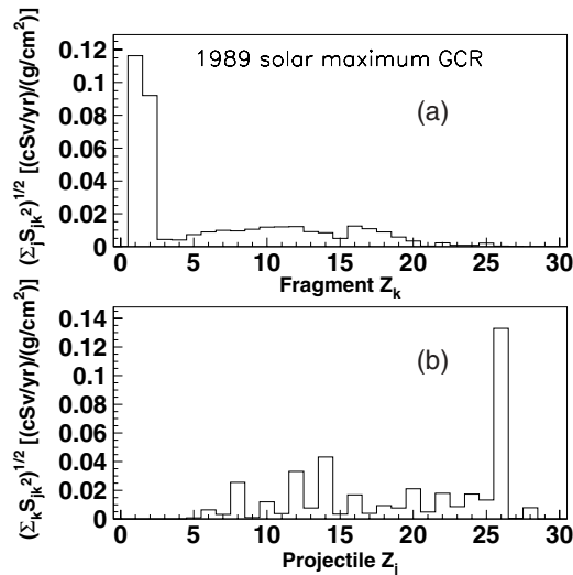
FIG. 10. Fragment (a) and projectile (b) distributions for the sensitivity of dose equivalent to a given relative change in the partial cross sections for the 1989 solar maximum GCR environment.
