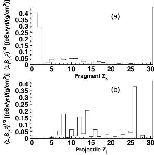
FIG. 3. Fragment (a) and projectile (b) distributions for the sensitivity of dose equivalent to a given relative change in the partial cross sections.
