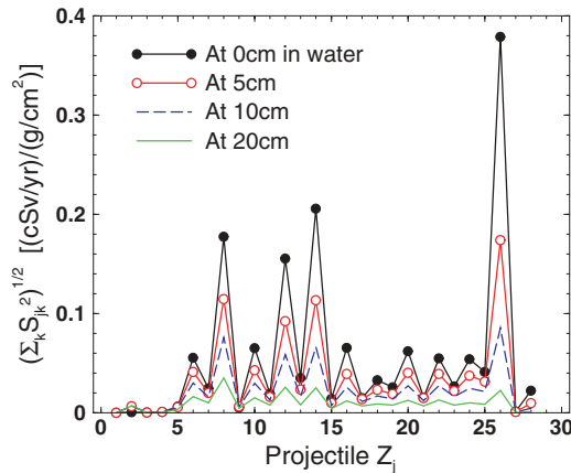
FIG. 6. (Color online) Projectile distributions for the sensitivity of dose equivalent at 0, 5, 10, and 20 g/cm 2 in water shielding to a given relative change in the partial cross sections.
