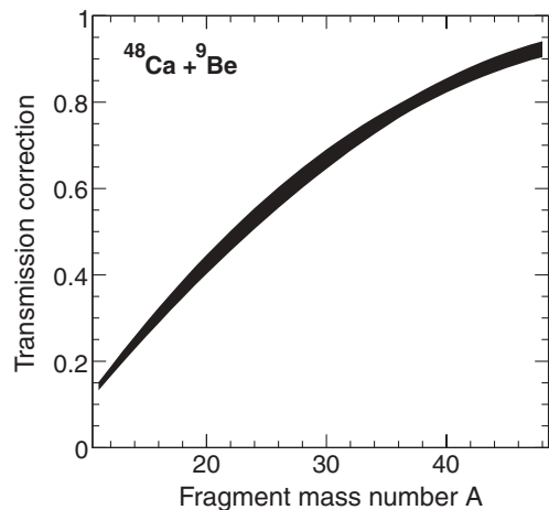
FIG. 3. Dependence of the transmission correction, \epsilon , on the fragment mass number, A , for 48 Ca+ 9 Be reactions.
