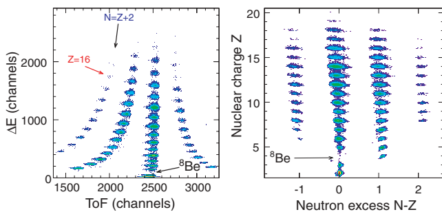
FIG. 2. (Color online) Raw (left panel) and calibrated (right panel) particle identification spectrum for 48 Ca+ 9 Be reactions at B\rho = 3.2 Tm.
