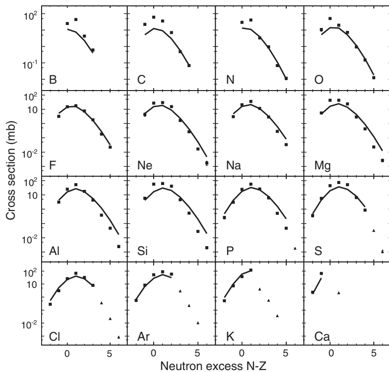
FIG. 7. Measured cross-sections presented as isotope distributions for 5 \leq Z \leq 20 elements detected in ^{40}\text{Ca}+^{181}\text{Ta} reactions at 140 MeV/nucleon. Experimental fragmentation data are shown as filled squares. Filled triangles show the cross-sections of nucleon pickup reactions. EPAX predictions are shown as solid lines.
