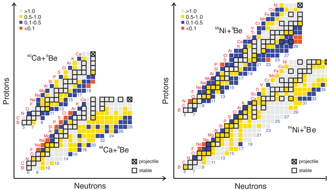
FIG. 14. (Color online) Ratios of measured fragment cross-sections and predicted cross-sections from EPAX parametrization for ^{40,48}\text{Ca} projectiles on ^9\text{Be} target (left panel) and ^{58,64}\text{Ni} projectiles on ^9\text{Be} target (right panel). The lightest grey color represents ratios with values greater than 1.
