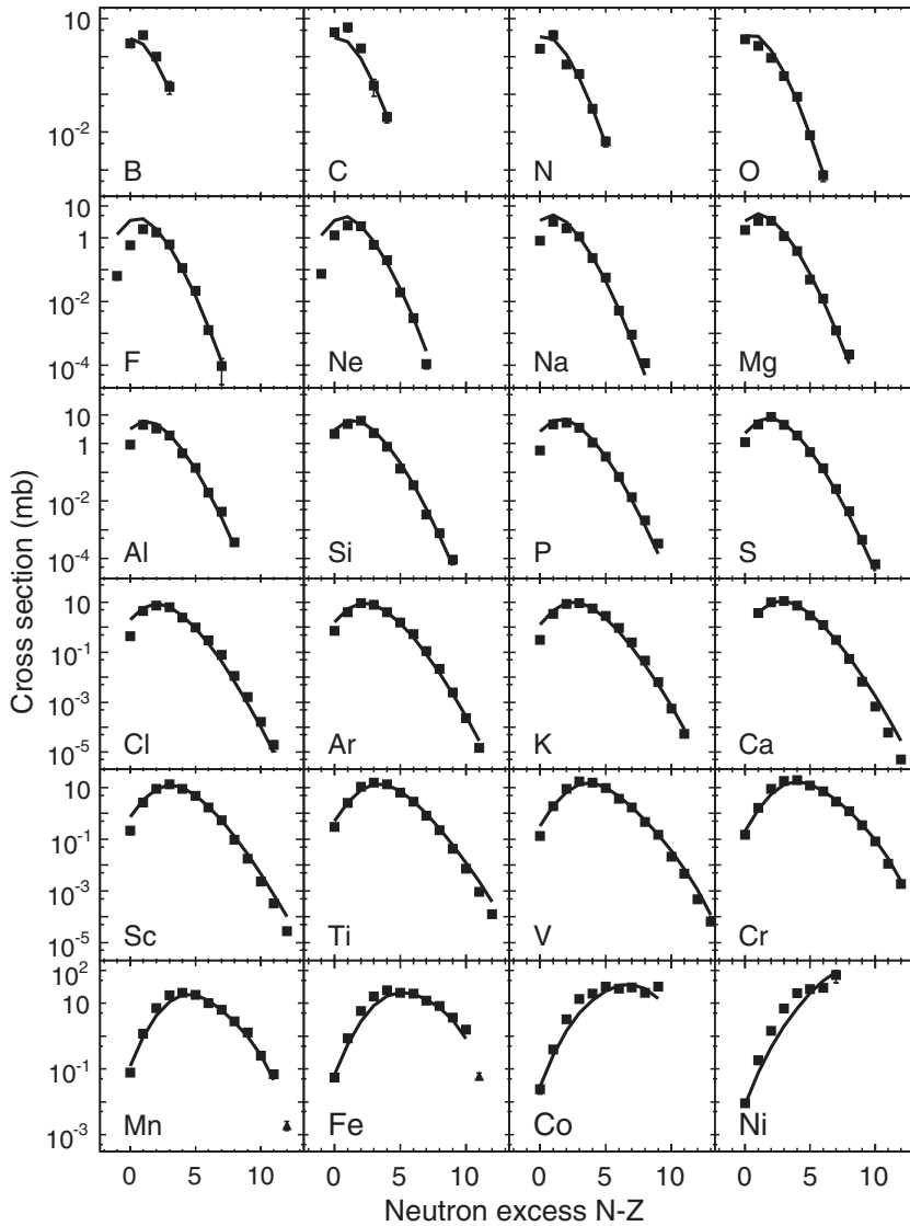
FIG. 12. Measured cross-sections presented as isotope distributions for 5 \leq Z \leq 28 elements detected in ^{64}\text{Ni}+^9\text{Be} reactions at 140 MeV/nucleon. Experimental fragmentation data are shown as filled squares. Filled triangles show the cross-sections of nucleon pickup reactions. EPAX predictions are shown as solid lines.
