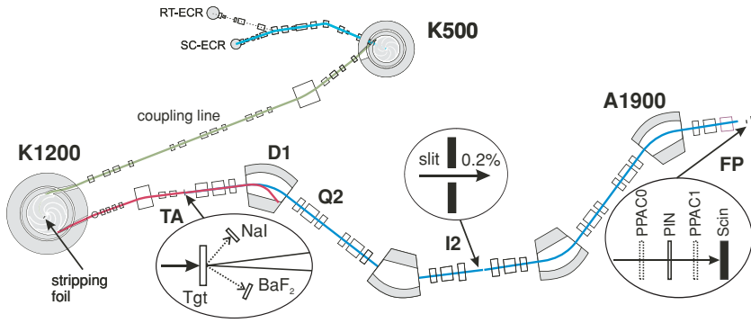
FIG. 1. (Color online) The A1900 fragment separator in stand-alone mode. Beam intensity monitors [NaI(Tl) and BaF 2 ] were located at the target station (TA). The momentum slit at the intermediate image (I2) defined the momentum opening (0.2% in dp/p ). The detector setup at the focal plane (FP) was used to identify fragments. The first dipole (out of four) is labeled D1 and the second quadrupole triplet (out of eight) is labeled Q2.
