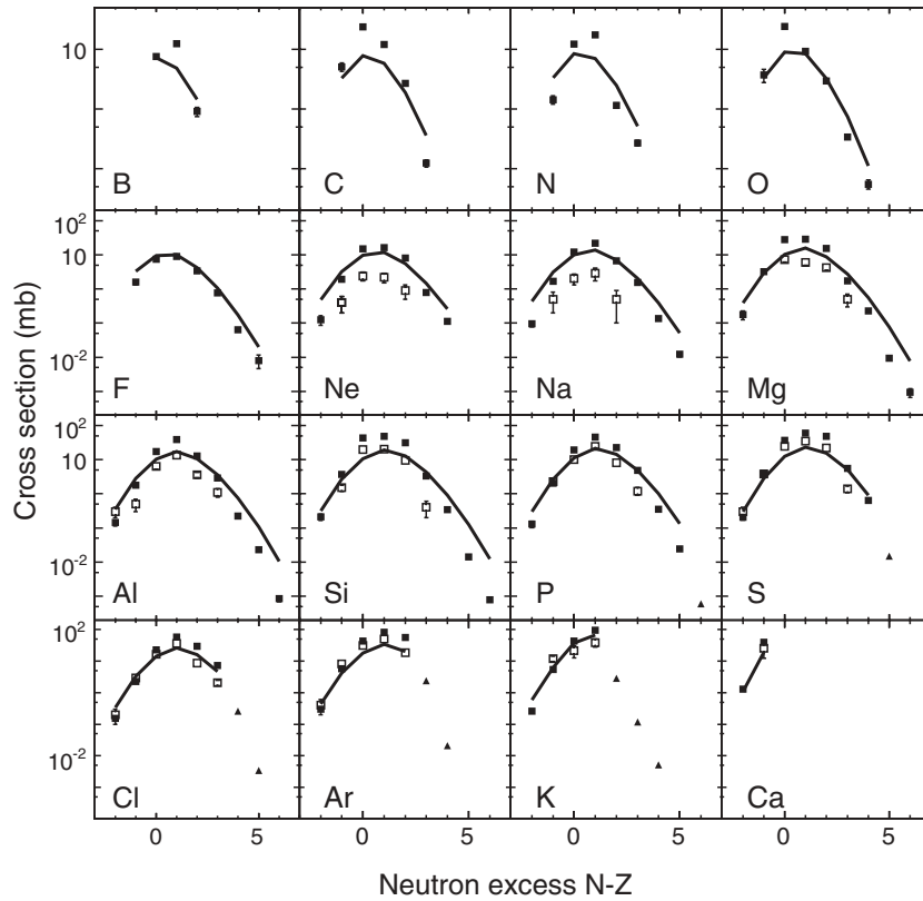
FIG. 6. Measured cross-sections presented as isotope distributions for 5 \leq Z \leq 20 elements detected in ^{40}\text{Ca}+^9\text{Be} reactions at 140 MeV/nucleon. Experimental fragmentation data are shown as filled squares. Filled triangles show the cross-sections of nucleon pickup reactions. EPAX predictions are shown as solid lines. Open squares show ^{40}\text{Ca}+^1\text{H} at 356 MeV/nucleon.
