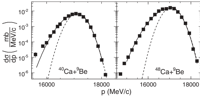
FIG. 4. Momentum distributions for ^{33}\text{P} produced in fragmentation of ^{40}\text{Ca} (left panel) and ^{48}\text{Ca} (right panel) primary beams. The solid curve represents a fit with Eq. (3) and the dotted curve is a Gaussian fit to the right side of the momentum distribution to show the asymmetry of the experimental distributions.
