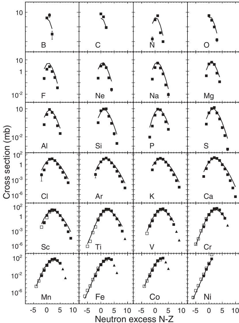
FIG. 10. Measured cross-sections presented as isotope distributions for 5 \leq Z \leq 28 elements detected in ^{58}\text{Ni}+^9\text{Be} reactions at 140 MeV/nucleon. Experimental fragmentation data are shown as filled squares. Filled triangles show the cross-sections of nucleon pickup reactions. EPAX predictions are shown as solid lines. Open squares show ^{58}\text{Ni}+^9\text{Be} at 650 MeV/nucleon [28].
