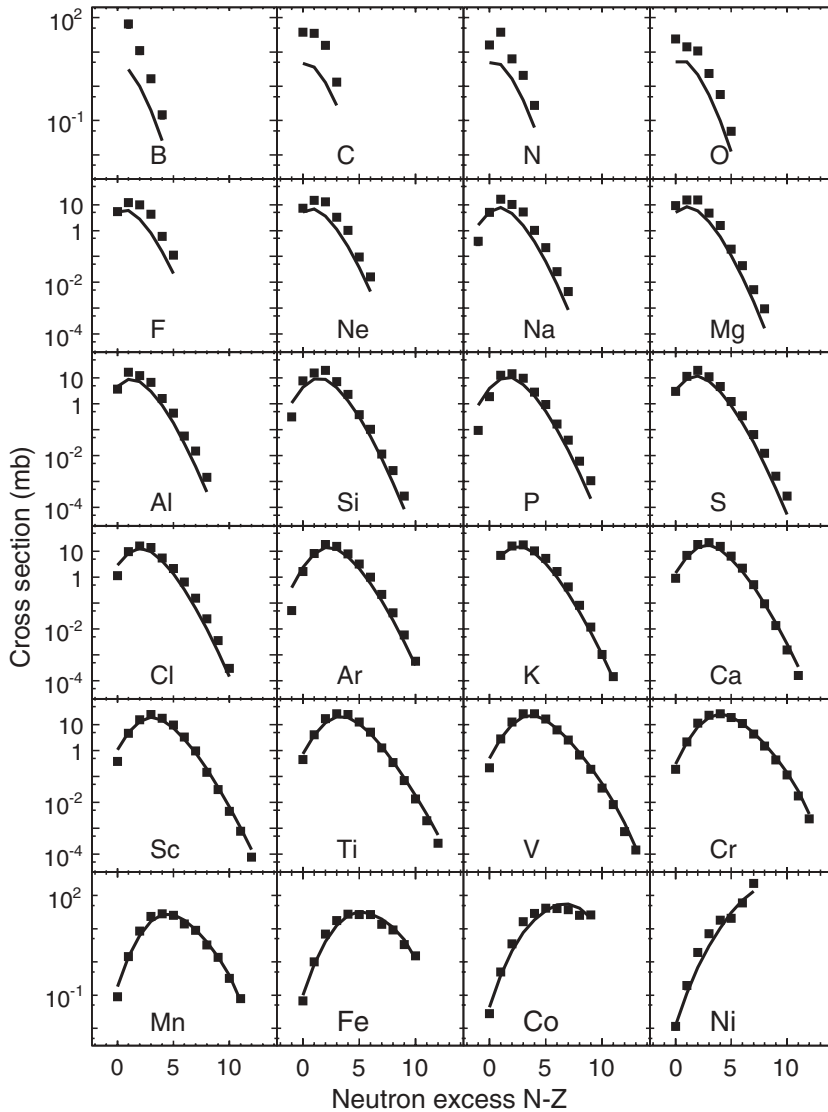
FIG. 13. Measured cross-sections presented as isotope distributions for 5 \leq Z \leq 28 elements detected in ^{64}\text{Ni} + ^{181}\text{Ta} reactions at 140 MeV/nucleon. Experimental fragmentation data are shown as filled squares. EPAX predictions are shown as solid lines.
