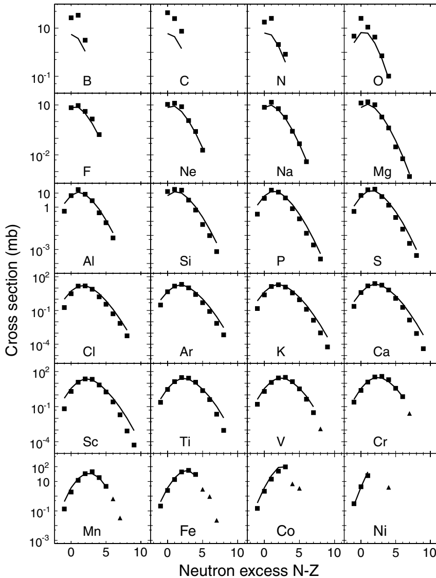
FIG. 11. Measured cross-sections presented as isotope distributions for 5 \leq Z \leq 28 elements detected in ^{58}\text{Ni}+^{181}\text{Ta} reactions at 140 MeV/nucleon. Experimental fragmentation data are shown as filled squares. Filled triangles show the cross-sections of nucleon pickup reactions. EPAX predictions are shown as solid lines.
