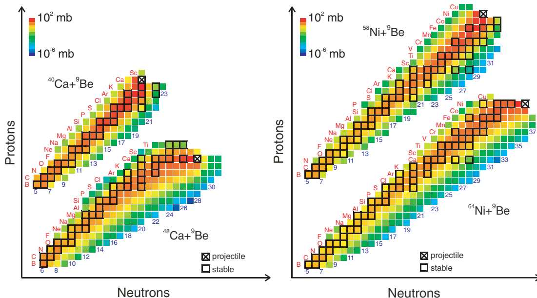
FIG. 5. (Color online) Isotope cross-sections measured in the fragmentation of ^{40,48}\text{Ca} projectiles on ^9\text{Be} target (left panel) and in the fragmentation of ^{58,64}\text{Ni} projectile on ^9\text{Be} target (right panel).
