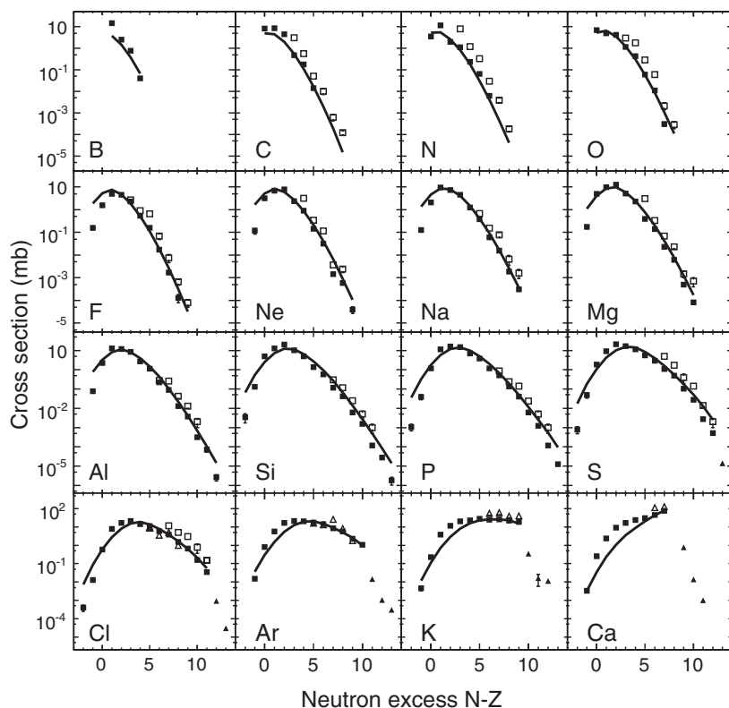
FIG. 8. Measured cross-sections presented as isotope distributions for 5 \leq Z \leq 20 elements detected in ^{48}\text{Ca}+^9\text{Be} reactions at 140 MeV/nucleon. Experimental fragmentation data are shown as filled squares. Filled triangles show the cross-sections of nucleon pickup reactions. EPAX predictions are shown as solid lines. Open squares show ^{48}\text{Ca}+^9\text{Be} at 212 MeV/nucleon [26]. Open triangles show fragments created in the ^{48}\text{Ca}+^2\text{H} at 104 MeV/nucleon [27].
