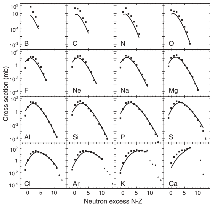
FIG. 9. Measured cross-sections presented as isotope distributions for 5 \leq Z \leq 20 elements detected in ^{48}\text{Ca}+^{181}\text{Ta} reactions at 140 MeV/nucleon. Experimental fragmentation data are shown as filled squares. Filled triangles show the cross-sections of nucleon pickup reactions. EPAX predictions are shown as solid lines.
