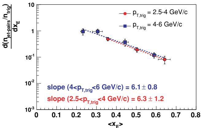
FIG. 31. (Color online) Conditional yield as a function of \langle x_E \rangle for the far-side h - h correlations for two trigger p_T ranges. Dashed lines are exponential fits to the data. Bars are statistical errors.
