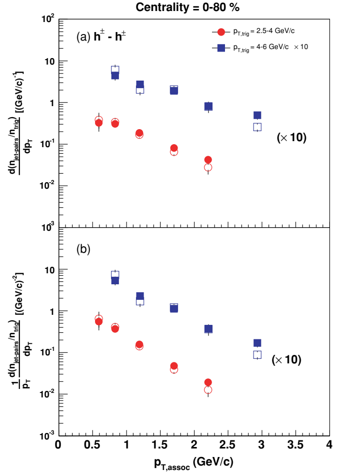
FIG. 20. (Color online) Per-trigger yield (a) and invariant conditional yield (b) as a function of p_{T,assoc} for the trigger hadron ranges shown. Closed points are the near-side yields; open points are the far-side yields. Centrality range is 0–80% in d + Au collisions. Yields are corrected for efficiency and reported in the PHENIX \eta acceptance. Bars are statistical errors.
