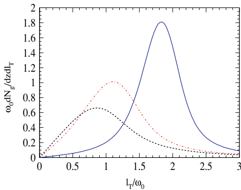
FIG. 1. (Color online) Gluon bremsstrahlung spectra induced by multiple parton scattering: \omega_0 dN_g/dz d\ell_T vs \ell_T/\omega_0 , where \omega_0 \equiv \sqrt{2Ez(1-z)/L} . Spectra are scaled by P(z)\tilde{C}\alpha_s^2 L m_N/\omega_0^2 , and the gluon fractional momentum is set z = 0.2 . Dashed line is for ordinary gluon bremsstrahlung with LPM interference as given by Eq. (1). Solid and dot-dashed lines are the distribution in Eq. (4) for the bremsstrahlung of gluons that has a space-like dispersion relation with -\Pi_T(\ell)/\omega_0^2 = 4 and 1, respectively.
