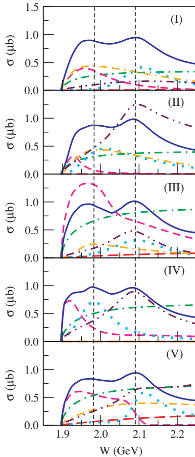
FIG. 8. (Color online) Total cross section for \gamma p \rightarrow p\eta' as a function of the total energy of the system, W = \sqrt{s} . The panels from top to bottom correspond to the fit results of Tables I–V, as indicated. The overall total cross sections (solid lines) are broken down according to their dynamical contributions, with line styles defined in Fig. 3. The two dashed vertical lines are placed to guide the eye through the two bump positions in all panels.
