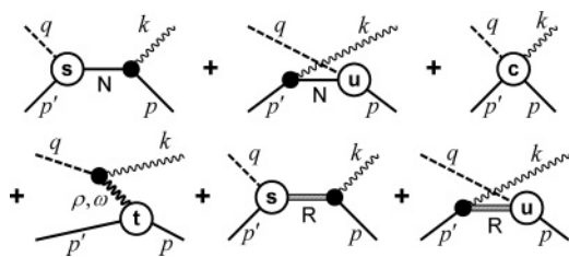
FIG. 1. Diagrams contributing to \gamma p \rightarrow \eta' p . Time proceeds from right to left. The intermediate baryon states are denoted N for the nucleon and R for the S_{11} , P_{11} , P_{13} , and D_{13} resonances. The intermediate mesons in the t -channel are \rho and \omega . The external legs are labeled by the four-momenta of the respective particles and the labels s , u , and t of the hadronic vertices correspond to the off-shell Mandelstam variables of the respective intermediate particles. The three diagrams in the lower part of the diagram are transverse individually; the three diagrams in the upper part are made gauge invariant by an appropriate choice for the contact current depicted in the top-right diagram. The nucleonic current (nuc) referred to in the text corresponds to the top line of diagrams; the meson-exchange current (mec) and resonance current contributions correspond, respectively, to the leftmost diagram and the two diagrams on the right of the bottom line of diagrams.
