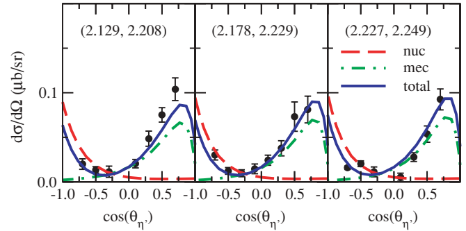
FIG. 9. (Color online) Fit result with no resonances. g_{NN\eta'} = 2.10 and \Lambda_v = 1264 MeV. See the legend to Fig. 3.
