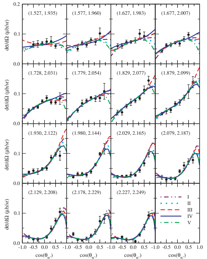
FIG. 2. (Color online) Differential cross section for \gamma p \rightarrow p\eta' according to the mechanisms shown in Fig. 1 as a function of the \eta' emission angle \theta_{\eta'} in the center-of-momentum frame of the system. As indicated in the legend, the curves correspond to the fit results of Tables I (dash-double-dotted), II (dotted lines), III (dashed), IV (solid), and V (dash-dotted). The numbers ( T_\gamma , W ) in parentheses are the incident photon energy T_\gamma and the corresponding s -channel energy W = \sqrt{s} , respectively, in GeV. The data are from Ref. [11].
