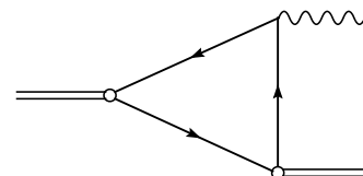
FIG. 1. Quark loop contribution to the radiative decay.
