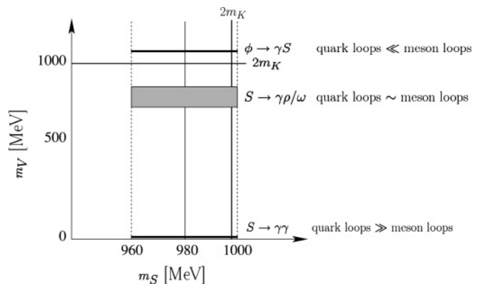
FIG. 5. Illustration of various kinematical regimes probed by the decays involving scalars.
