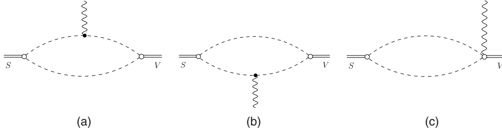
FIG. 3. Meson loop contributions to the radiative decay of scalar mesons. Diagram (c) is required to provide the overall gauge invariance of the amplitude.
