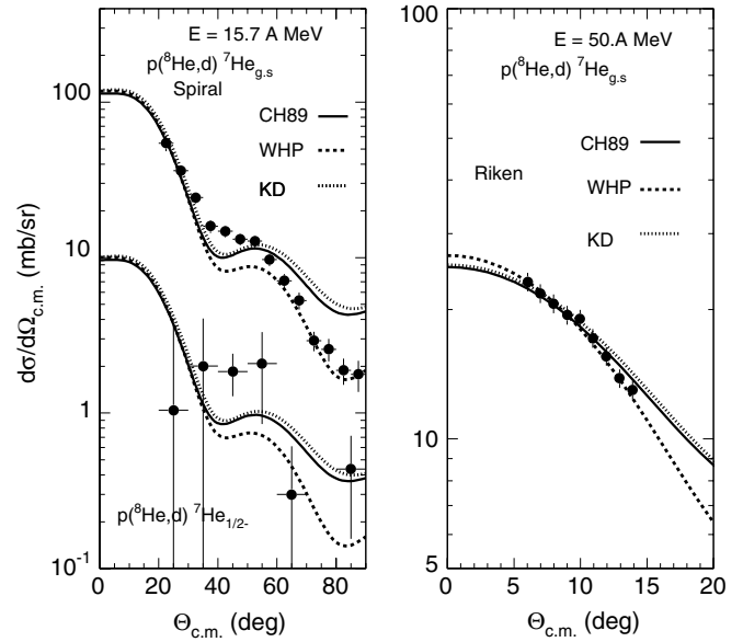
FIG. 7. Analysis of the (p, d) cross sections to {}^7\text{He}_{\text{g.s.}} and {}^7\text{He}_{1/2^-} obtained at 15.7 and (p, d){}^7\text{He}_{\text{g.s.}} at 50A MeV [5].
