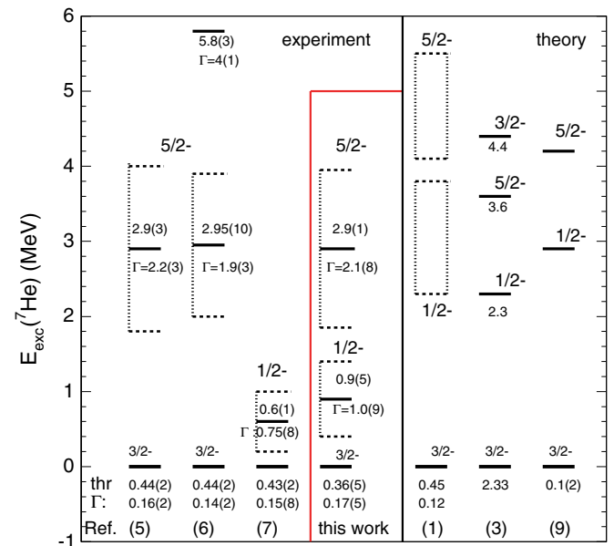
FIG. 8. (Color online) Experimental and theoretical spectra of {}^7\text{He} . The threshold energy indicated for the models is deduced from the predicted binding energy for {}^7\text{He} and the energies of the excited states are given with respect to the calculated g.s.
