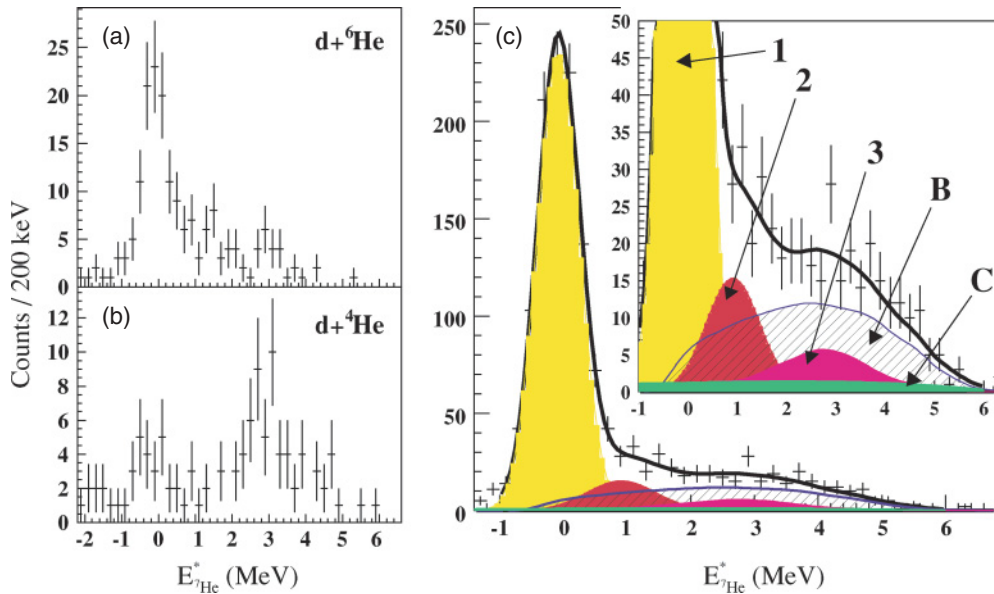
FIG. 4. (Color online) Excitation spectra for ^7\text{He} with following conditions (see also the text): (a) coincidence with the deuteron and the ^6\text{He} fragment in the plastic wall; (b) coincidence with the ^4\text{He} ; (c) the areas 1 and 2, 3, B and C correspond to the resonances for the g.s. and two excited states, to the physical and carbon backgrounds, respectively. The thick solid curve is the total fit including all contributions. The error bars on the points are statistical errors. The insert shows a zoom.
