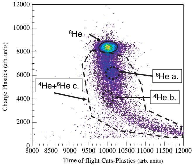
FIG. 3. (Color online) Correlation spectrum of the charge in the plastic wall versus TOF. The data correspond to the events of ^8\text{He} on proton, for which a light charged particle ( p , d , or triton) was detected in MUST. TOF is between the second beam detector CATS and the plastics. The contours (gates) indicated in the plot are discussed in the text.
