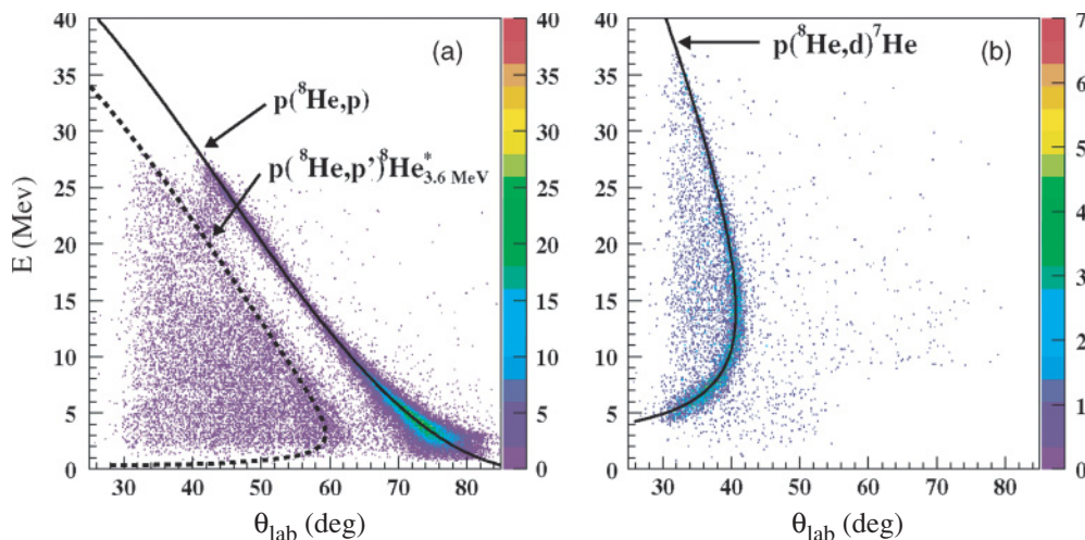
FIG. 2. (Color online) Kinematical plot of events for: (a) the ^8\text{He} elastic, inelastic reactions on protons and (b) ( p, d ) transfer. The calculated lines of the reactions are drawn to guide the eye, the dashed line in (a) represents the ( p, p' ) to an excited state at 3.6 MeV.
