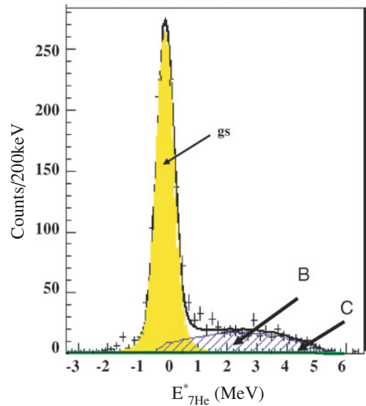
FIG. 6. (Color online) Excitation spectrum for {}^7\text{He} . Areas B and C correspond to the physical and carbon backgrounds, respectively. The thick solid curve is the total fit including g.s. resonance and all contributions. The error bars on the points are statistical errors.
