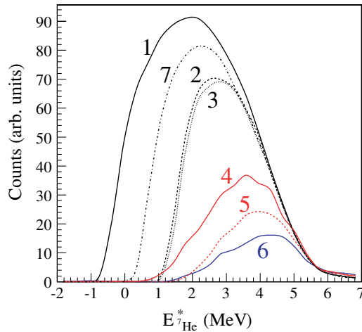
FIG. 5. (Color online) Physical background contributions expressed as a function of the excitation energy for {}^7\text{He} . Each curve is obtained by simulation of the various reaction channels detailed in the text.
