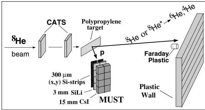
FIG. 1. Experimental setup. The MUST array was assembled in a wall configuration, located 15 cm from the target. It was placed in two positions with the vertical axis rotated by an angle of 50^\circ and 65^\circ with respect to the beam axis in the laboratory frame.
