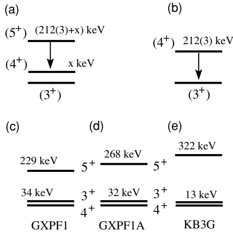
FIG. 3. Two possible scenarios (a) and (b) for the placement of the 212(3)-keV transition in the decay scheme of ^{52}\text{Sc} compared with shell model calculations (c)–(e). An E2 transition from the 5^+ to the 3^+ level can be excluded as discussed in the text.
