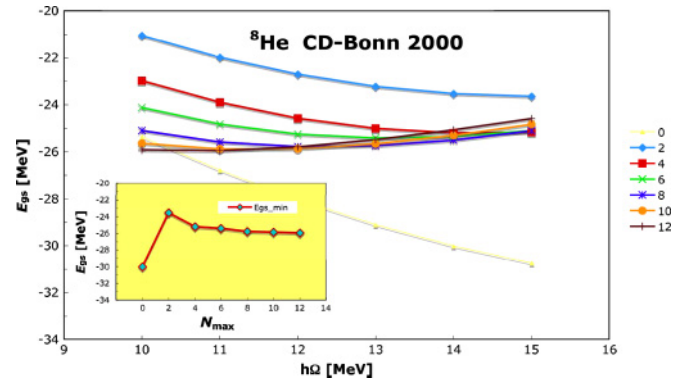
FIG. 3. (Color online) The same as in Fig. 1, but for ^8\text{He} and model spaces from N_{\text{max}} = 0 to N_{\text{max}} = 12 .
