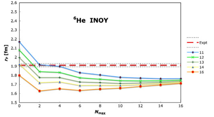
FIG. 7. (Color online) The same as in Fig. 5, but for the INOY NN potential and HO frequencies from \hbar\Omega = 11 MeV to \hbar\Omega = 16 MeV.
