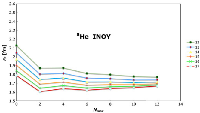
FIG. 9. (Color online) The same as in Fig. 8, but for the INOY NN potential and HO frequencies from \hbar\Omega = 12 MeV to \hbar\Omega = 17 MeV.
