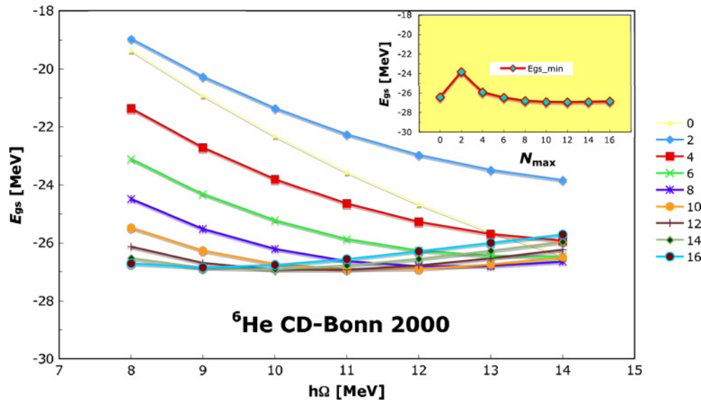
FIG. 1. (Color online) The {}^6\text{He} ground-state energy dependence on the HO frequency for different model-spaces sizes from N_{\text{max}} = 0 to N_{\text{max}} = 16 obtained using the CD-Bonn 2000 NN potential. The inset demonstrates how the values at the minima of each curve converge with increasing N_{\text{max}} .
