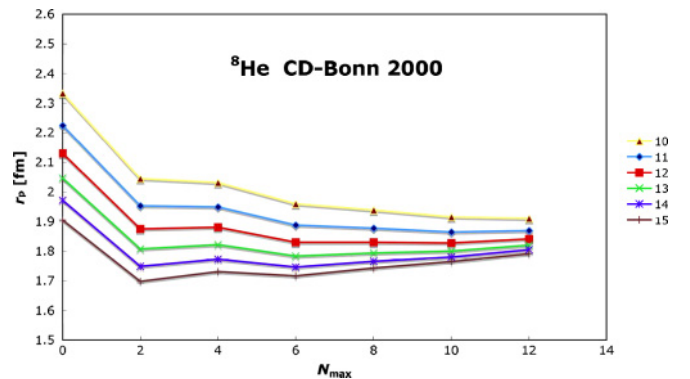
FIG. 8. (Color online) The {}^8\text{He} point-proton rms radius dependence on the model space size for different HO frequencies from \hbar\Omega = 10 MeV to \hbar\Omega = 15 MeV obtained using the CD-Bonn 2000 NN potential.
