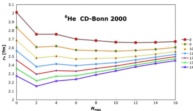
FIG. 6. (Color online) The {}^6\text{He} point-neutron rms radius dependence on the model space size for different HO frequencies from \hbar\Omega = 8 MeV to \hbar\Omega = 14 MeV obtained using the CD-Bonn 2000 NN potential.
