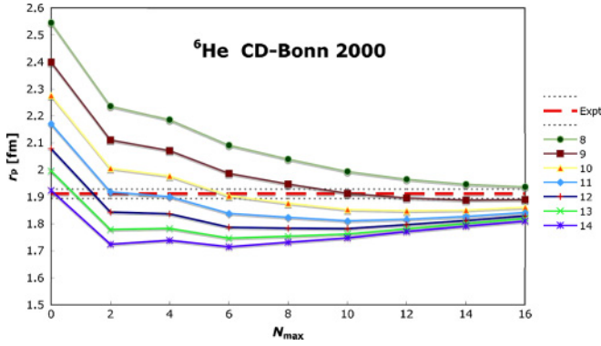
FIG. 5. (Color online) The {}^6\text{He} point-proton rms radius dependence on the model space size for different HO frequencies from \hbar\Omega = 8 MeV to \hbar\Omega = 14 MeV obtained using the CD-Bonn 2000. The experimental value is from Ref. [2].
