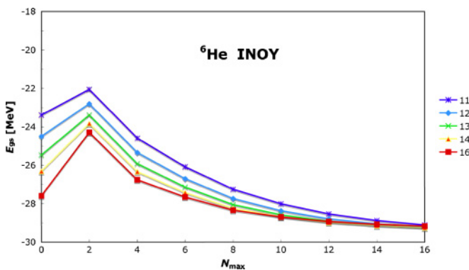
FIG. 2. (Color online) The ^6\text{He} ground-state energy dependence on the model space size for different HO frequencies from \hbar\Omega = 11 MeV to \hbar\Omega = 16 MeV obtained using the INOY NN potential.
