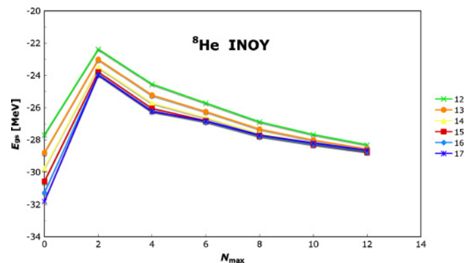
FIG. 4. (Color online) The same as in Fig. 2, but for ^8\text{He} and HO frequencies from \hbar\Omega = 12 MeV to \hbar\Omega = 17 MeV.
