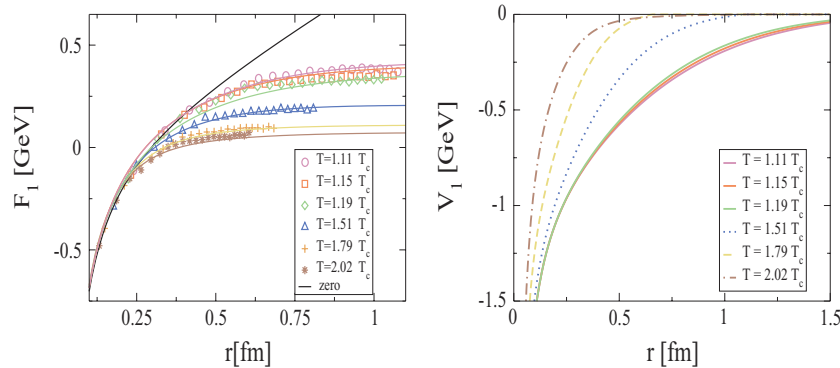
FIG. 1. (Color online) Left panel: Lattice QCD results for the color-singlet free energy from unquenched simulations [27] for six different values of the temperature (symbols) compared to our fit function, Eq. (1), represented by the various curves. Right panel: Corresponding potential in the color-singlet channel obtained with Eq. (5) for the six different values of the temperature.
