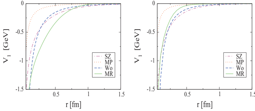
FIG. 2. (Color online) Comparison of Q\text{-}\bar{Q} color-singlet potentials as determined from various lattice data in our (MR) and other works (SZ [21], MP [18], and Wo [17]); the left (right) panel is for T = 1.5T_c ( 2T_c ).
