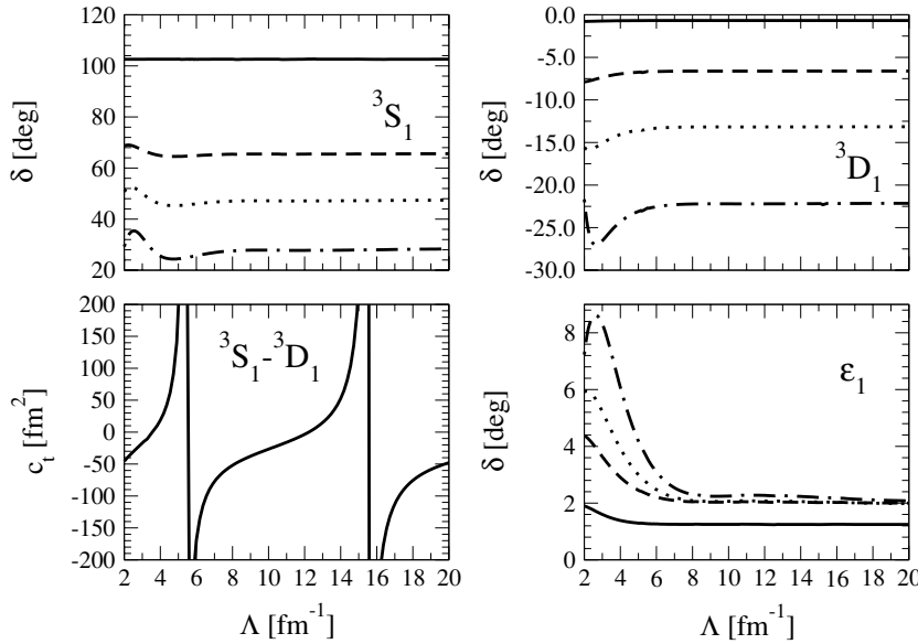
FIG. 2. Fit result for the counterterm c_i as a function of the cutoff, and the resulting cutoff dependence of the {}^3S_1 - {}^3D_1 phase shifts and the mixing angle \epsilon_1 at laboratory energies of 10 MeV (solid line), 50 MeV (dashed line), 100 MeV (dotted line), and 190 MeV (dash-dotted line).
