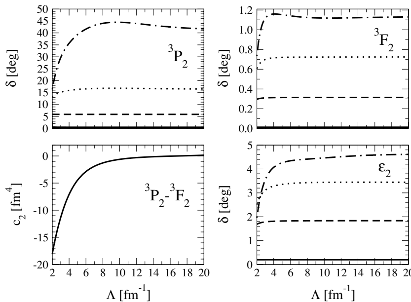
FIG. 11. Fit result for the counterterm c_2 as a function of the cutoff, and the resulting cutoff dependence of the {}^3P_2 - {}^3F_2 phase shifts and the mixing angle \epsilon_2 at laboratory energies of 10 MeV (solid line), 50 MeV (dashed line), 100 MeV (dotted line), and 190 MeV (dash-dotted line).
