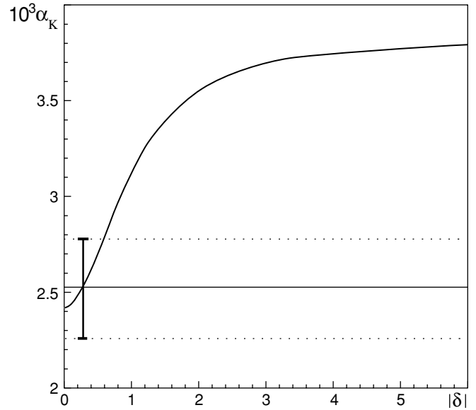
FIG. 5. The calculated value of \alpha_K as a function of |\delta| is compared to the experimental one for the 453 keV transition deexciting the 3024 keV level. The error bar corresponds to one standard deviation.
