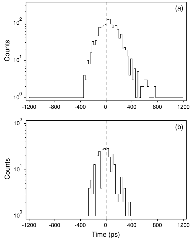
FIG. 4. Time-delayed \beta\gamma(t) spectra gated by the fast response \beta and BaF 2 detectors with the following gates: \beta -917(Ge)-424(BaF 2 ) in the top panel and \beta -1263(Ge)-424(BaF 2 ) in the bottom panel. The difference in the centroids is due to the lifetime of the 0 + 770 keV level. The broken line marks the centroid of the bottom spectrum, from which the centroid of top spectrum is visibly shifted to the right. The observed time-shift is 51(18) ps and it corresponds to a half-life of the 770 keV level of 35(12) ps; see text for discussion. Time scale is 26.1 ps/ch.
