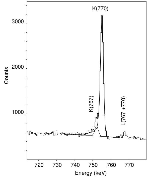
FIG. 6. Relevant section of an electron-energy spectrum showing the K - and L -conversion lines of the 770 keV, 0_2^+ \rightarrow 0_1^+ transition. The two close lying K -770 keV and K -767 keV transitions (the latter deexcites the 3024 keV level) are clearly resolved by the fitting procedure.
