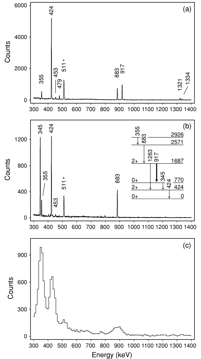
FIG. 2. Selected results from the \beta\gamma\gamma coincidences using \beta -Ge-Ge and \beta -Ge-BaF 2 detectors. Top panel: portion of the Ge energy spectrum in coincidence with the 345 keV transition. Middle and bottom panels: portion of the coincident Ge and BaF 2 energy spectra, respectively, gated on the 917 keV transition in Ge. The latter spectrum shows good separation of the 345, 424, 511, and 883 keV peaks. This is crucial in order to select the 345–424, 917–424, 917–345 time-delayed coincidences, which were used to determine the lifetime of the 0^+ 770 keV level; see text for details.
