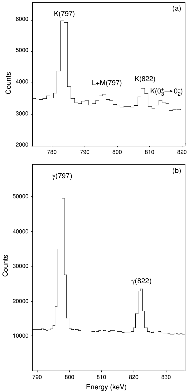
FIG. 7. Relevant sections of electron (a) and \gamma (b) energy spectra showing the region around 800 keV. In the electron spectrum, in addition to the conversion lines of the 797 keV, 2_2^+ \rightarrow 2_1^+ transition and 822 keV transition, deexciting the 2104 keV level, a line at 814 keV is present with no counterpart in the \gamma spectrum. It has been identified as the K -conversion line of the 0_3^+ \rightarrow 0_2^+ transition (see text).
