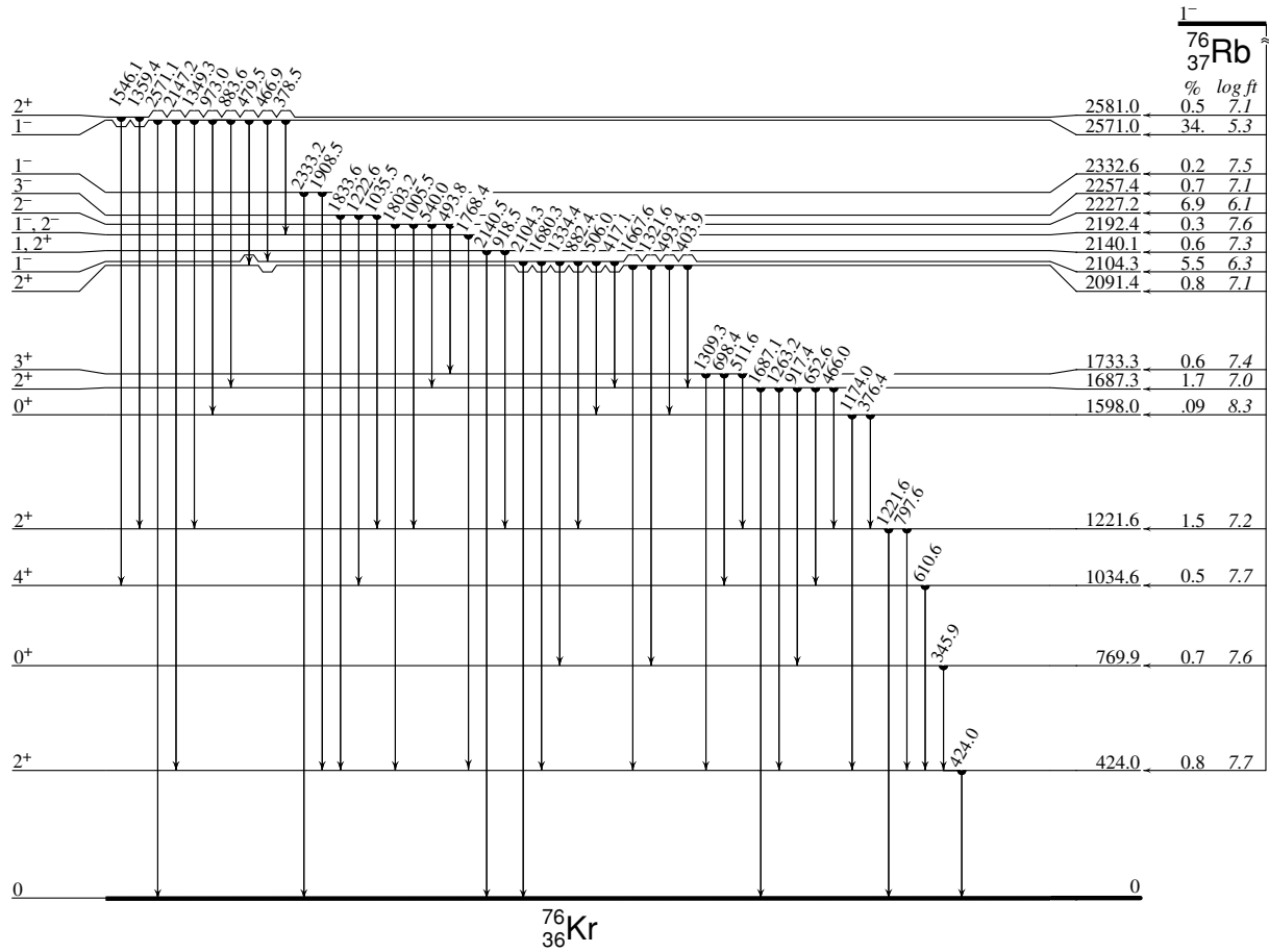
FIG. 8. Partial level scheme of ^{76}\text{Kr} showing the decay of the states populated in the \beta^+ -decay of ^{76}\text{Rb} . The feeding percentage and the associated \log ft values are reported on the right-hand side of the figure up to 2600 keV.
