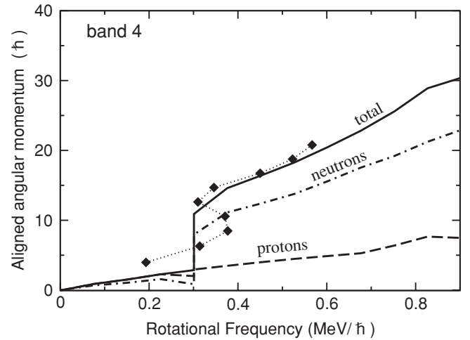
FIG. 5. Experimental data points, connected by a dotted guideline, and the calculated alignment curves for the \pi g_{7/2} band. The dot-dashed and dashed curves correspond to contributions to the aligned angular momentum emanating from the neutrons and proton orbitals, respectively.
