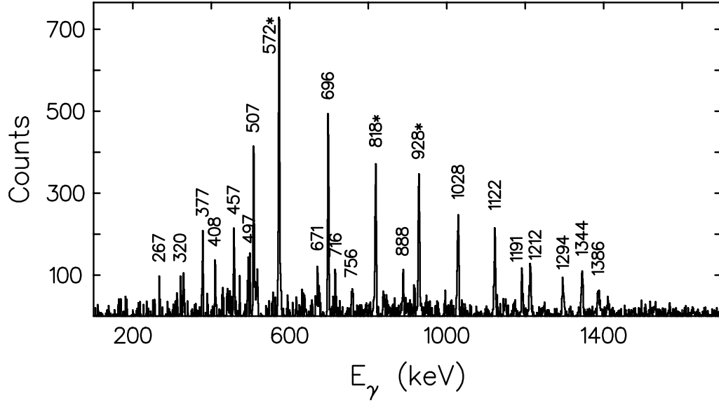
FIG. 2. Sum of \gamma -ray spectra gated by the members of the band 3. Gating transitions are marked with an asterisk symbol.
