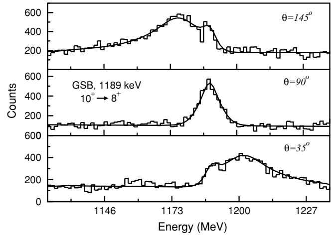
FIG. 6. Lineshape fit in ^{76}\text{Kr} for the ground-state band transition, 1189 keV, from the backed-target data. The top, middle, and bottom panels correspond to lineshapes at the mean angles 145^\circ, 90^\circ, and 35^\circ , respectively.
