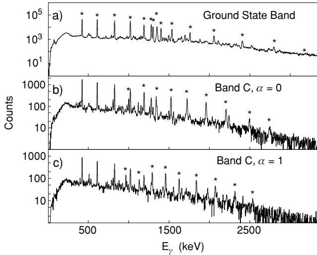
FIG. 1. \gamma -ray spectra obtained by summing pairs of double coincidence gates set on in-band transitions in (a) the ground-state band of ^{76}\text{Kr} , (b) the \alpha = 0 signature of Band C, and (c) the \alpha = 1 signature of Band C. In each case, the in-band transitions are denoted by an asterisk.
