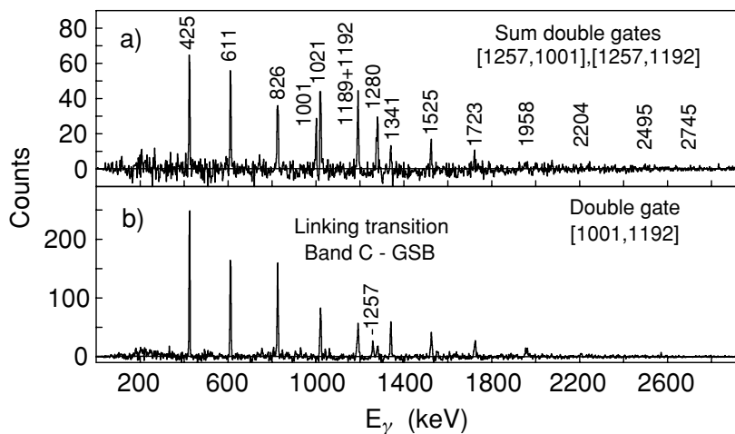
FIG. 4. Upper panel shows the sum of the background subtracted \gamma -ray spectrum in coincidence with a double gate set on the 1001- and 1192-keV transitions in Band C and the 1257-keV linking transition. Lower panel shows the background subtracted \gamma -ray spectrum in coincidence with a double gate set on the 1001- and 1192-keV transitions in Band C. The 1257-keV transition links Band C and the ground-state band (GSB).
