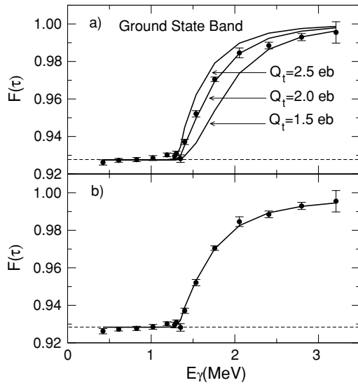
FIG. 5. Experimental F(\tau) values as a function of \gamma -ray energy for the ground-state band (filled circles) in ^{76}\text{Kr} . The solid lines in plot (a) show the calculated F(\tau) values for various constant transition quadrupole moments ( Q_t = 1.5, 2.0, and 2.5 e b ). The solid line in plot (b) shows the calculated F(\tau) value, considering that Q_t varies as a function of spin (see text). The dashed line represents the F(\tau) value reached by the recoils that leave the target.
