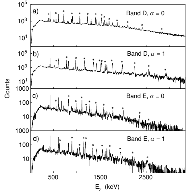
FIG. 2. \gamma -ray spectra obtained by summing pairs of double coincidence gates set on in-band transitions in (a) the \alpha = 0 signature of Band D, (b) the \alpha = 1 signature of Band D, (c) the \alpha = 0 signature of Band E, and (d) the \alpha = 1 signature of Band E. In each case, the in-band transitions are denoted by an asterisk.
