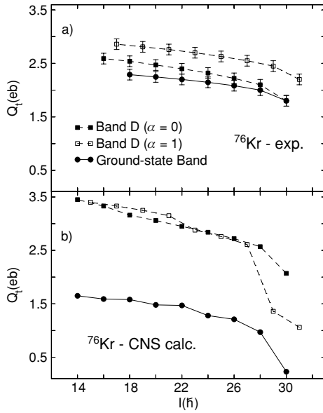
FIG. 12. Top panel shows the measured transition quadrupole moments Q_t for the ground-state band and Band D. Lower panel shows the calculated Q_t values for the [2,4] and [3,4] configurations that are interpreted as the ground-state band and Band D, respectively.
