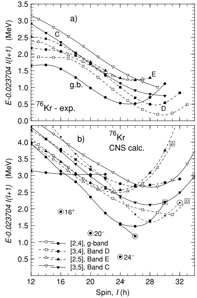
FIG. 10. Energies of high-spin collective configurations in ^{76}\text{Kr} relative to an I(I + 1) reference plotted versus spin from (a) experiment and (b) configuration-dependent cranked Nilsson-Strutinsky calculations. Solid (dashed) lines represent positive (negative) parity, and closed (open) symbols denote signature \alpha = 0 ( \alpha = 1 ). In panel (b) terminating states are circled, whereas the maximum spin states that do not terminate are indicated by large squares. The calculated bands are labeled by [p, n] , where p(n) is the number of g_{9/2} protons (neutrons). The band label has been added next to the assigned configuration. A second even spin [3,4] configuration lower in energy for the spin range I \approx 25\text{--}30 is shown by a thinner line and smaller closed squares. Note that the absolute normalization for experiment and calculations is different
