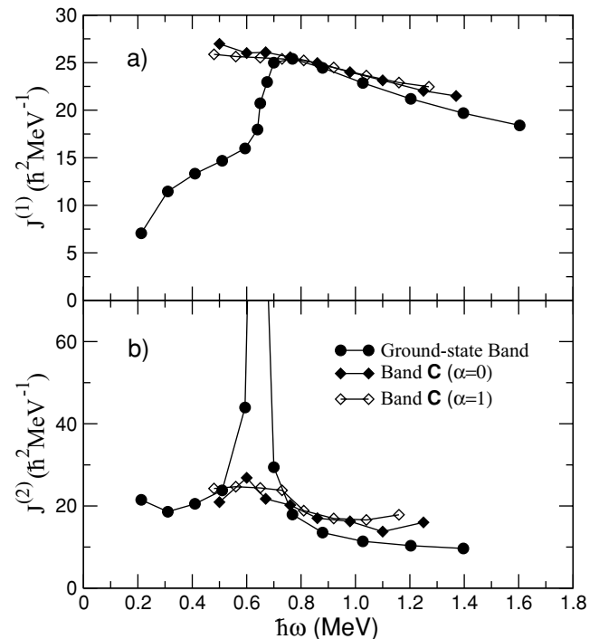
FIG. 7. (a) Kinematic and (b) dynamic moments of inertia for the ground-state band and Band C in ^{76}\text{Kr} plotted versus rotational frequency.
