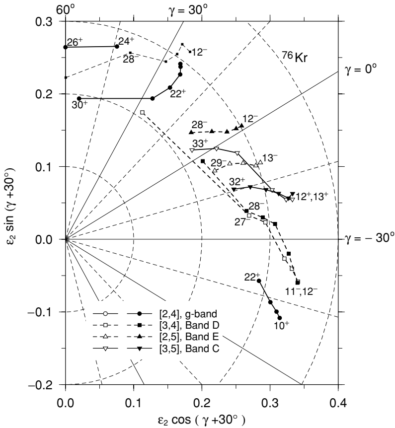
FIG. 11. Calculated deformation trajectories for ^{76}\text{Kr} . The deformations are shown for each fourth spin value except for the band terminating at I^\pi = 26^+ , where the I^\pi = 24^+ state is also shown.
