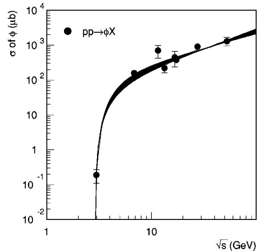
FIG. 14. Parametrization of the \phi yield in p+p interactions. The data points are from Refs. [5,48,56]. The fit is discussed in the text.
