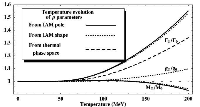
FIG. 2. Temperature evolution of the \rho mass, width, and \rho\pi\pi coupling. The dashed line corresponds to Eq. (7), the dotted line to the real axis IAM, Eq. (4), and the solid line is the IAM pole position. The M_0, \Gamma_0, g_0 values are given in the text.
