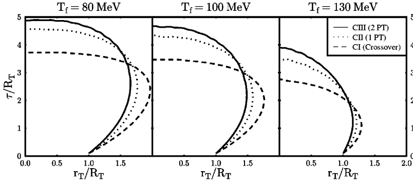
FIG. 4. Hypersurfaces T=T_f for the three chiral EOS. This figure corresponds to initial conditions as appropriate for central Au+Au collisions at BNL-RHIC energy ( \sqrt{s}=130A GeV).
