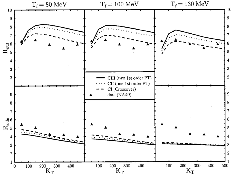
FIG. 5. R_{\text{side}} and R_{\text{out}} as a function of K_T at SPS. T_f=80,100,130 MeV.
