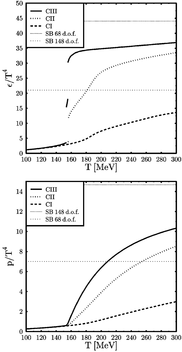
FIG. 1. \epsilon/T^4 and p/T^4 for the three different parameter sets CI, CII, CIII at \mu_q = \mu_s = 0 . Depending on the chosen parameters we observe a different phase transition behavior. For CI a smooth crossover occurs. In contrast CII leads to a jump in \epsilon/T^4 at T \approx 150 MeV and a discontinuity in the rise of p/T^4 with T . Finally, CIII even shows two discontinuities in \epsilon/T^4 . The horizontal lines correspond to the Stefan-Boltzmann limit with and without the (anti)baryon decuplet.
