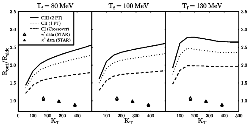
FIG. 8. R_{\text{out}}/R_{\text{side}} as a function of K_T at RHIC.
