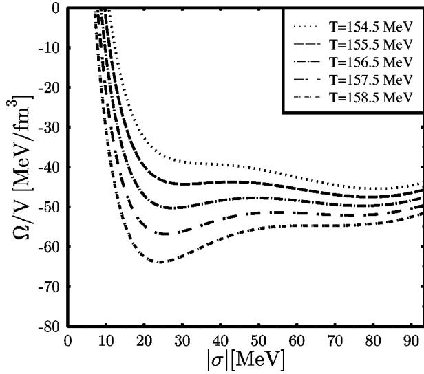
FIG. 3. Effective potential \Omega/V \equiv -p as a function of the scalar condensate \sigma around T_c . For parameter set CII and \mu_q = \mu_s = 0 ( \zeta has been chosen such as to maximize the pressure for given \sigma ).
