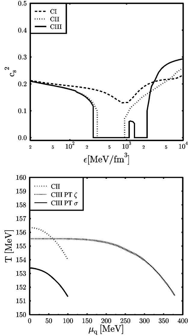
FIG. 2. Top: c_s^2 \equiv \partial p / \partial \epsilon for three different equations of state at \mu_q = \mu_s = 0 . Bottom: Phase diagram for the parameter sets CII and CIII for f_s \equiv \rho_s / \rho_B = 0 . The two chemical potentials ( \mu_q, \mu_s ) of the system lead to a slight change of the temperature in the phase transition region.
