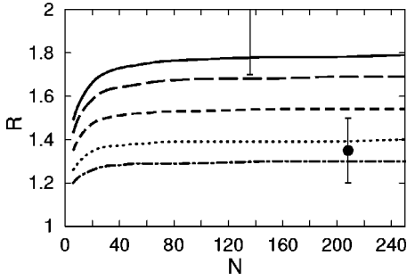
FIG. 5. The exact result for the ratio R as a function of N at \chi = 0.8 (solid line), 0.7 (long dashed line), 0.55 (short dashed line), 0.4 (dotted line), and 0.3 (dash-dotted line). The full circle with error bar at N=208 is the experimental value of R obtained for DGDR in ^{208}\text{Pb} . The experimental value of R for DGDR in ^{136}\text{Xe} is shown by the vertical line at N=136 , whose center at R=2.4 is beyond the scale.
