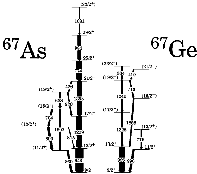
FIG. 6. Comparison of high-spin states built on the 9/2^+ isomer in ^{67}\text{As} (left) and ^{67}\text{Ge} (right).
