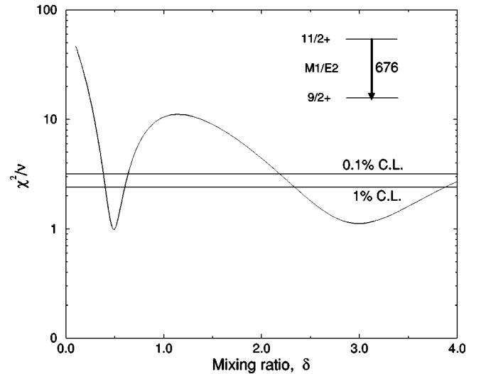
FIG. 5. \chi^2 per degree of freedom for various values of mixing ratio delta for the 676-keV M1/E2 transition in ^{69}\text{Se} . The initial alignment parameter, \sigma/J for the fit was 0.54. The 1% and 0.1% confidence limits are indicated.
