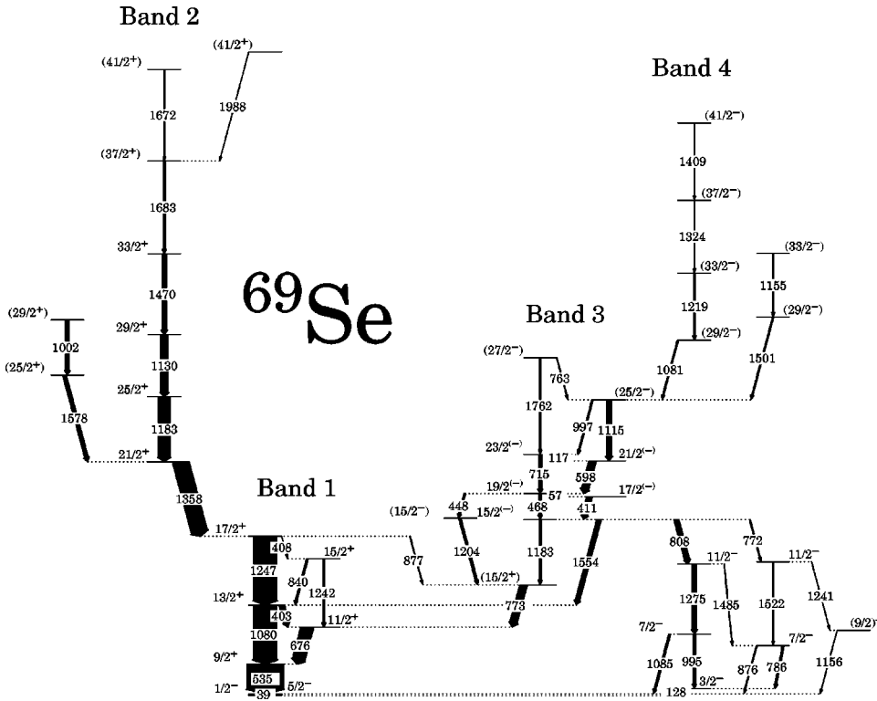
FIG. 2. Partial level scheme for ^{69}\text{Se} . The width of the arrows is proportional to the intensity of the transitions.
