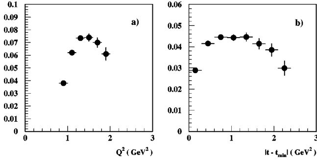
FIG. 7. Acceptance as a function of Q^2 and -t' .
