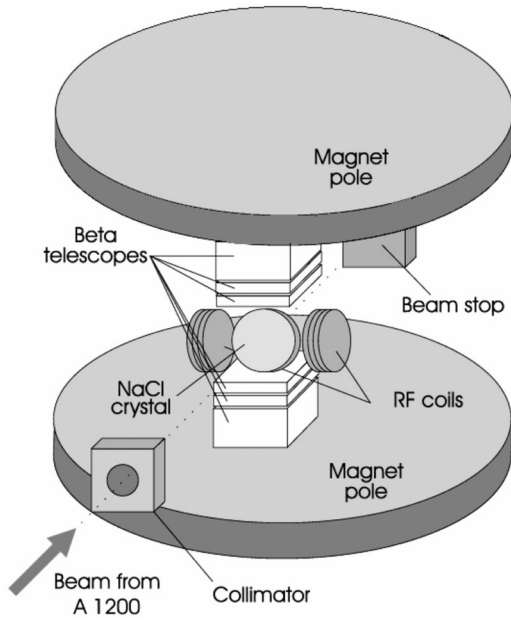
FIG. 1. Schematic of the NSCL \beta -NMR apparatus.
