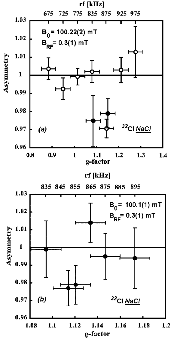
FIG. 2. Resonance curves obtained for ^{32}\text{Cl} implanted in \text{NaCl} . The applied frequency modulation was (a) \pm 25 kHz and (b) \pm 10 kHz. The rf modulation had a ramp waveform with a 500 Hz repetition rate.
