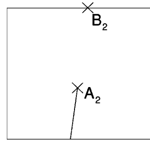
FIG. 1. Phase diagram for one \bar{\phi}_i field coupled to a SU(3) gauge field. In Figs. 1 and 2, the y axis is \lambda , from 0 to \infty , and the x axis is \sim m_\phi^2 .
