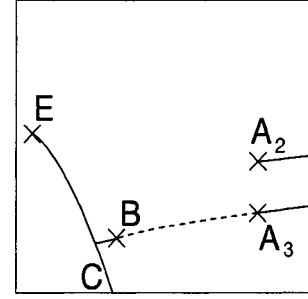
FIG. 4. Cartoon of the QCD phase diagram in the large gap limit.
