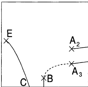
FIG. 3. Cartoon of the QCD phase diagram in the small gap limit. In Figs. 3 and 4, the y axis is temperature, and the x axis is quark chemical potential.
