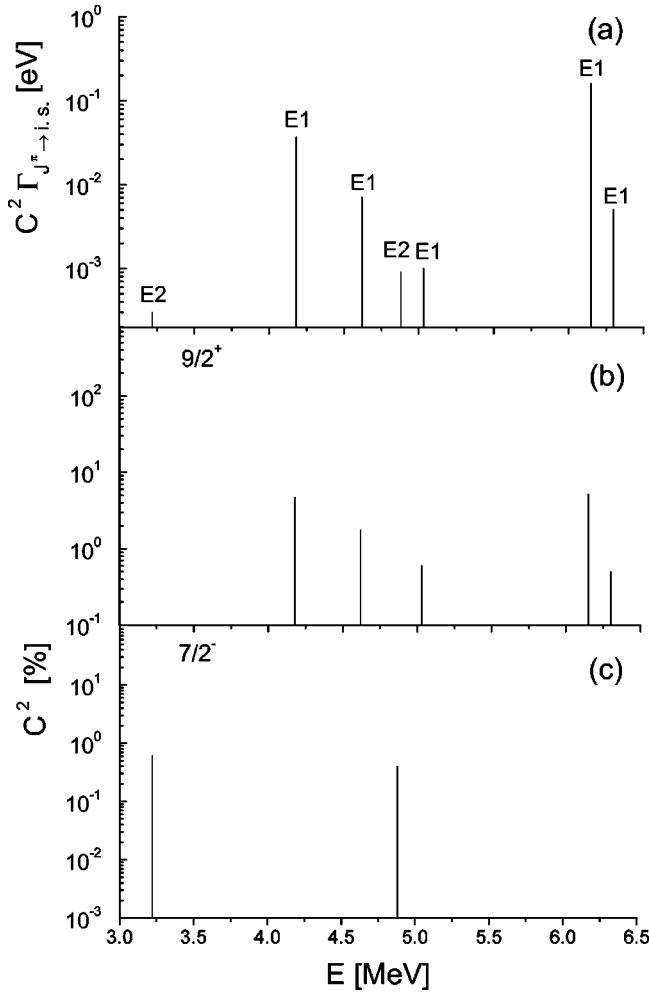
FIG. 3. (a) Decay probability C^2\Gamma for population of the isomeric state in ^{139}\text{Ce} from excited states at intermediate energies; (b),(c) contribution of one-quasiparticle configuration C^2 to wave functions of decaying states with different spin and parity. The multipolarity of each transition is indicated on top of lines in (a). J^\pi of decaying states is specified in (b) and (c).
