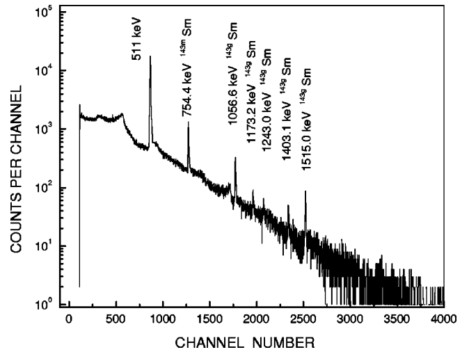
FIG. 1. \gamma -ray spectrum measured after activation of ^{144}\text{Sm} target by bremsstrahlung radiation with endpoint energy E_{\gamma_{\text{max}}} = 25 MeV. The \gamma -lines used in the data analysis are indicated for the isomeric and ground states.
