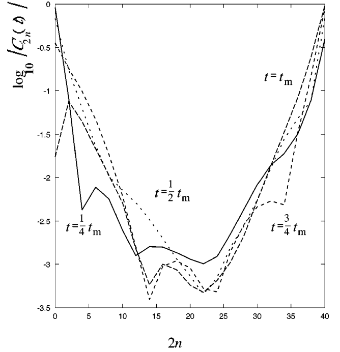
FIG. 5. The calculated logarithmic absolute values \log_{10}|c_{2n}(t)| of the expansion coefficients of the nuclear state |\check{\Psi}(0),t\rangle=\sum_n c_{2n}(t)|\check{\Psi}(2n)\rangle in terms of the mean-field states |\check{\Psi}(2n)\rangle at time t=t_1=\frac{1}{4}t_m (solid line), t_2=\frac{1}{2}t_m (dotted line), t_3=\frac{3}{4}t_m (short dashed line), and t_4=t_m (dashed line), where t_m=\pi/(E_{19}-E_{20})=7\,750\,981\,924\,759.3\pi . The parameters used in this calculation are shown in the text.
