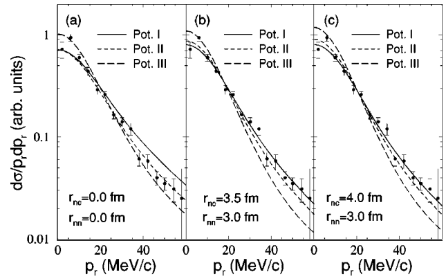
FIG. 3. Radial neutron momentum distribution after fragmentation of ^{11}\text{Li} on a carbon target at 280 MeV/nucleon. Core diffraction is not included. The experimental data from [10] is compared with calculations using the potentials I (solid), II (short-dashed), and III (long-dashed) in Table I. The shadowing parameters are given in the figure. The optical model parameters are from [28].
