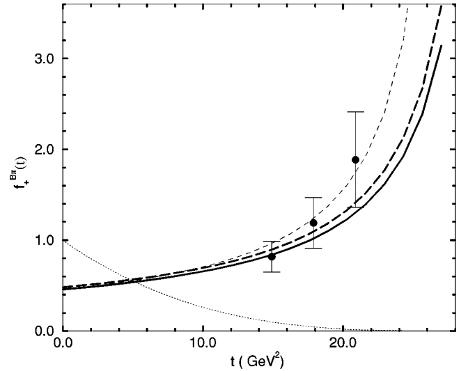
FIG. 1. Our calculated form of f_+^{B\pi}(t) : solid line, column 1, Table I; dashed line, column 2, Table I. For comparison, the data are the results of a lattice simulation [25] and the light, short-dashed line is a vector dominance, monopole model: f_+(t) = 0.46/(1-t/m_{B^*}^2) , m_{B^*}=5.325 GeV. The light, dotted line is the phase space factor |f_+^{B\pi}(0)|^2[(t_+-t)(t-t_-)]^{3/2}/(\pi m_B)^3 in Eq. (11), which illustrates that the B \rightarrow \pi e \nu branching ratio is determined primarily by the small- q^2 behavior of this form factor.
