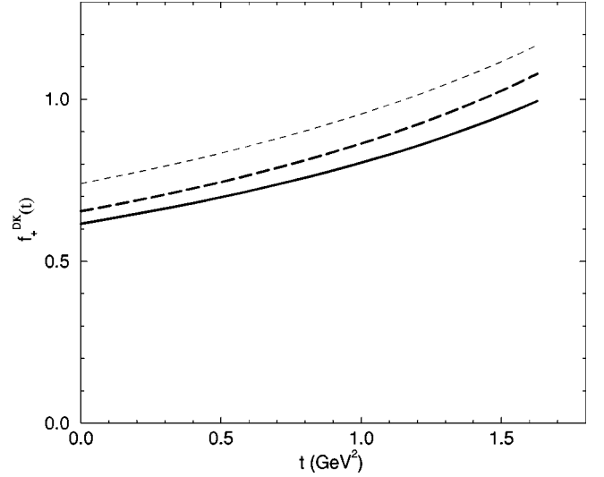
FIG. 3. Our calculated form of f_+^{DK}(q^2) : solid line, column 1, Table I; dashed line, column 2, Table I. For comparison the light, short-dashed line is a vector dominance, monopole model: f_+(q^2) = 0.74/(1 - q^2/m_{D_s^*}^2) , m_{D_s^*} = 2.11 GeV.
