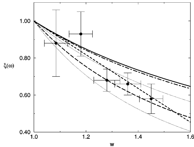
FIG. 2. A comparison of our calculated form of \xi(\omega) with recent experimental analyses. Our results: solid line, column 1, Table I; dot-dashed line, column 2, Table I. Experiment: data points, Ref. [28]; short-dashed line, linear fit from Ref. [29]; see our Eq. (54); long-dashed line, nonlinear fit from Ref. [29]; see our Eq. (55). The two light, dotted lines are this nonlinear fit evaluated with the extreme values of \rho^2 : upper line, \rho^2 = 1.17 , and lower line, \rho^2 = 1.89 .
