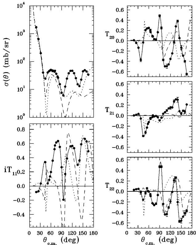
FIG. 5. Differential cross section and the four analyzing powers for {}^6\text{Li} - {}^4\text{He} elastic scattering at E_{\text{Li}}=19.6 MeV, with optical model calculations using parameter set 2 (dashed lines) and parameter set 3 (dotted lines) of Ref. [3].
