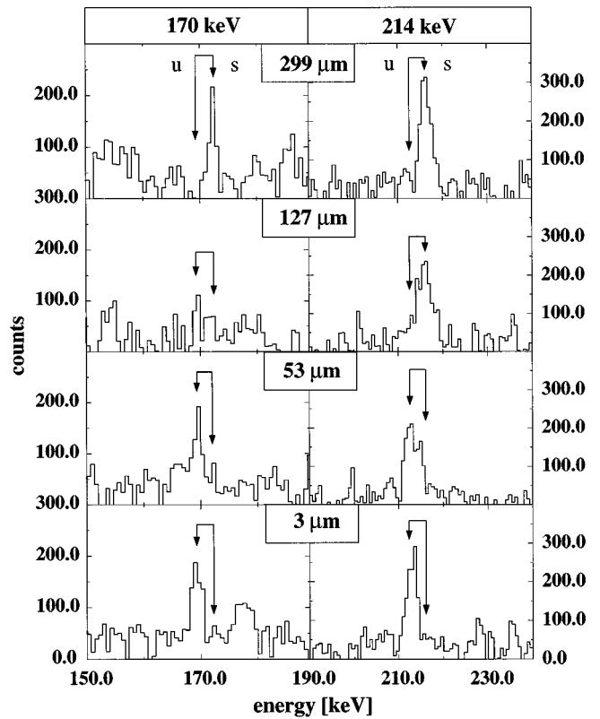
FIG. 2. As Fig. 1 for the 170 keV and 214 keV SD transitions, however, for a different set of distances. The spectra shown for the target-to-stopper distance of 299 \mu\text{m} are the sum of the statistics from the four longer distances at 299, 473, 700, and 1200 \mu\text{m} .
