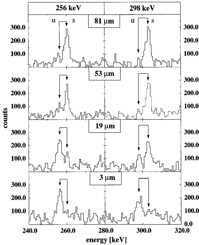
FIG. 1. Double gated spectra for the 256 keV and 298 keV SD transitions in ^{194}\text{Pb} at four different target-to-stopper distances (approximate distances from electrical contact are given in the insets). The spectra include the statistics of all detectors with considerable Doppler-shift (see text for details of the spectra manipulation). The unshifted (u) and Doppler-shifted (s) components of the transitions are marked.
