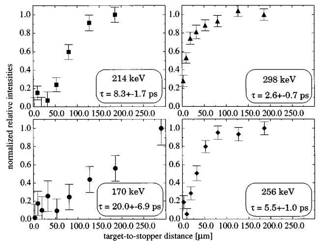
FIG. 3. Intensities of the Doppler-shifted component of the 170-, 214-, 256-, and 298-keV SD transitions as a function of the target-to-stopper distance. The intensities are normalized to the same number of events per distance and to the intensity at the largest distance.
