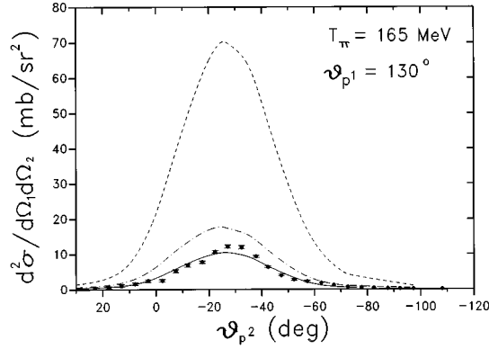
FIG. 3. Double differential cross section of the ^{12}\text{C}(\pi^+, pp)^{10}\text{B} reaction. The angle of proton 1 is fixed at \theta_{p1} = 130^\circ . The cross section is plotted versus the angle of proton 2. The data have been taken from Refs. [28,29]. The dashed curve shows the result with V_{\Delta N, \Delta N} = 0 while the dot-dashed curve shows the result with V_{\Delta N, \Delta N} \neq 0 . The solid curve shows the result with additional inclusion of the distortion of the decay protons.
