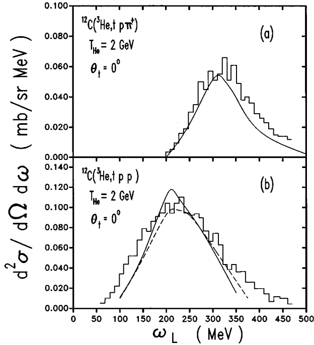
FIG. 5. Coincidence spectra for the ^{12}\text{C}(^3\text{He},t) reaction at T_{\text{He}} = 2 GeV and triton scattering angle \theta_i = 0^\circ . (a) The ^{12}\text{C}(^3\text{He},tp\pi^+) data [2] in comparison with the result of our calculation. (b) The ^{12}\text{C}(^3\text{He},tpp) reaction data [2]. The solid and dashed curve show the results with and without inclusion of the residual interaction, respectively.
