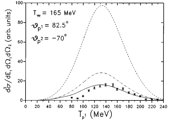
FIG. 4. Threefold differential cross section of the ^{12}\text{C}(\pi^+, pp)^{10}\text{B} reaction. The two protons were detected at \theta_{p1} = 82.5^\circ and \theta_{p2} = -70^\circ , respectively. The cross section is plotted as function of the kinetic energy of proton 1. The data have been taken from Refs. [28,29]. The curves shown have the same meaning as in Fig. 3. Note that the data are given in arbitrary units and are thus normalized to the solid curve.
