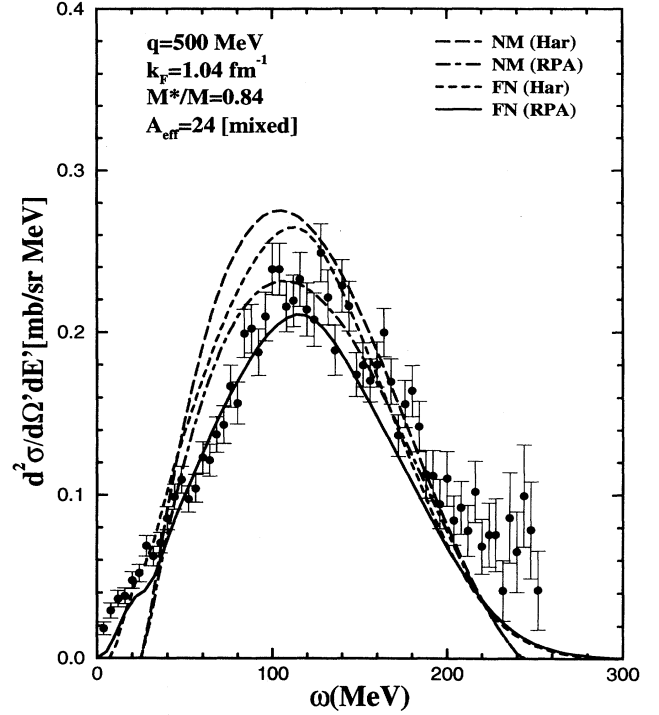
FIG. 4. Same as Fig. 3 except that the mixed representation of the K^+N amplitude is used and that the calculations are normalized using A_{\text{eff}} = 24 , the upper limit of the experimentally determined range of A_{\text{eff}} for ^{40}\text{Ca} [9, 10].
