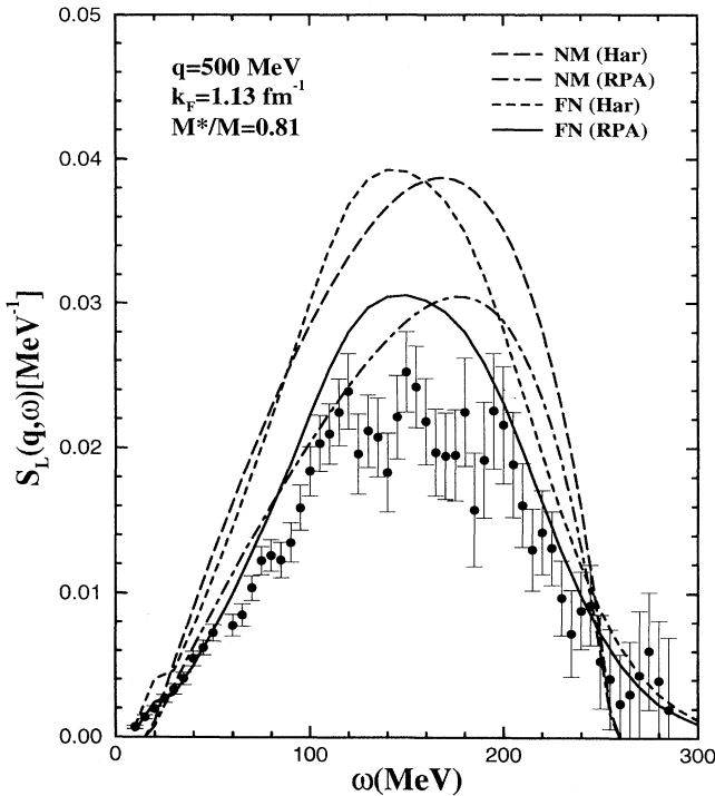
FIG. 1. The longitudinal ( e, e' ) response S_L for ^{40}\text{Ca} at |\mathbf{q}| = 500 \text{ MeV}/c . Data are from Ref. [1]. RHA nuclear matter (NM) and finite nucleus (FN) calculations without (Har) and with (RPA) RPA correlations as described in the text are shown.
