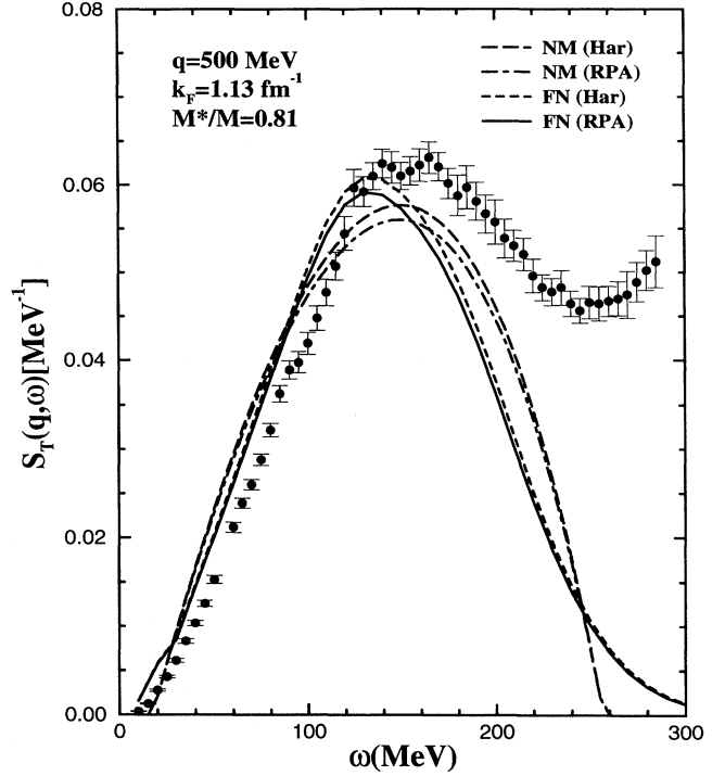
FIG. 2. Same as Fig. 1, but for the transverse ( e, e' ) response S_T .
