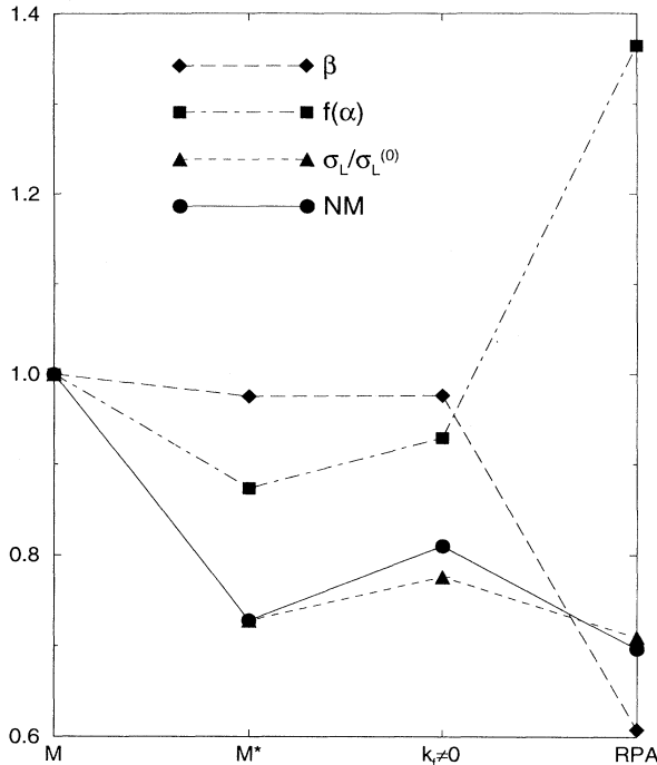
FIG. 5. The evolution of the integrated longitudinal isoscalar K^+ cross section per nucleon is shown for (i) a single nucleon of mass M initially at rest, (ii) a single nucleon of mass M^* = 0.81M initially at rest, (iii) a Fermi gas of nucleons of mass M^* = 0.81M and Fermi momentum k_F = 1.13 \text{ fm}^{-1} , and (iv) a system like (iii) except with RPA correlations. See discussion in text.
