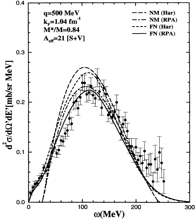
FIG. 3. The K^+ quasielastic cross section for ^{40}\text{Ca} at p_K = 703 \text{ MeV}/c and \theta_{\text{lab}} = 43^\circ . The data are from Refs. [9, 10]. RHA nuclear matter (NM) and finite nucleus (FN) calculations without (Har) and with (RPA) RPA correlations and employing the VS representation of the K^+N amplitude are shown. The calculations are normalized using A_{\text{eff}} = 21 , the centroid of the experimentally determined range of A_{\text{eff}} for ^{40}\text{Ca} [9, 10].
