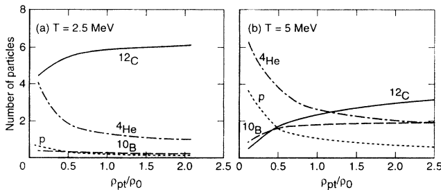
FIG. 1. Distribution of most abundant particles up to densities of 2.5\rho_0 . Curves for temperatures of 2.5 and 5 MeV are displayed. Other species have abundances which are smaller than the lowest curve shown here.
