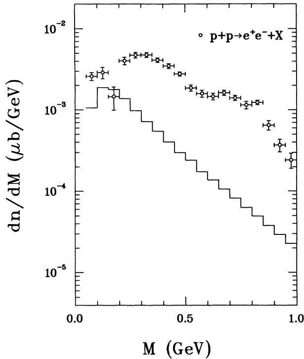
FIG. 8. The sum of bremsstrahlung contributions from NN , NN\pi , NN\pi\pi , and NN\pi\pi\pi final states in pp scattering. Data are again pp results from the Bevalac.
