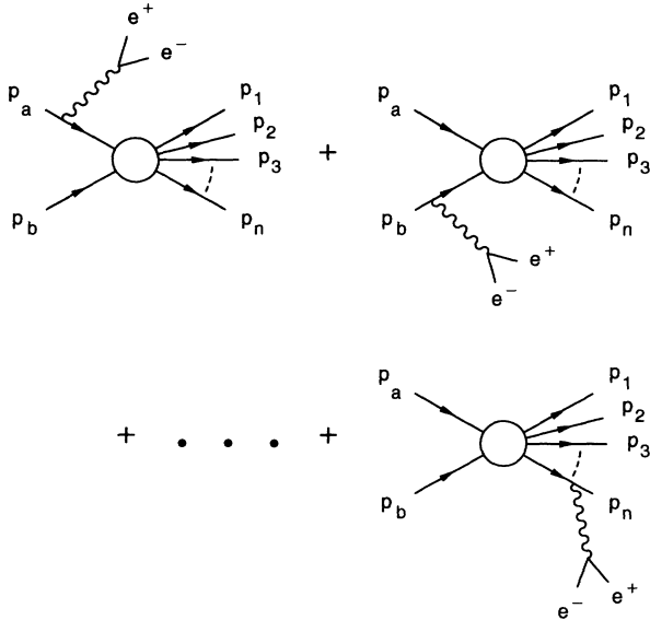
FIG. 1. Hadron-hadron collision with an n -particle final state where the arrows indicate momentum flow. A coherent sum of radiation for all charged external lines is computed.
