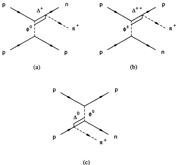
FIG. 5. Pion production diagrams proceed through \Delta^+ formation and decay as in (a), through \Delta^{++} formation and decay as in (b) and through \Delta^0 excitation as in (c). The exchanged meson \phi might be a pion, a rho meson, or some other boson.
