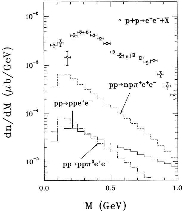
FIG. 6. Dilepton yields obtained from NN \rightarrow NN\pi bremsstrahlung as compared with simple nucleon-nucleon bremsstrahlung, and with pp data.
