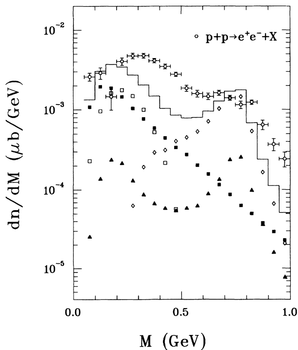
FIG. 9. Dilepton yields from various mechanisms: bremsstrahlung is presented as solid squares, radiative decay of the \Delta is presented as solid triangles, Dalitz decay of the \eta is shown as open squares, two-pion annihilation is shown as open diamonds, and finally, the sum of all contributions shown as the solid histogram.
