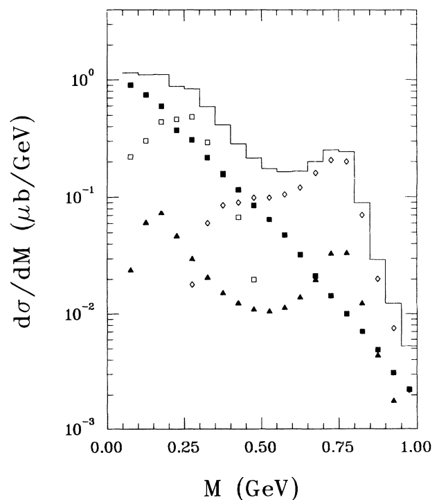
FIG. 10. Cross section (invariant mass distributions) from various mechanisms: bremsstrahlung is presented as solid squares, radiative decay of the \Delta is presented as solid triangles, Dalitz decay of the \eta is shown as open squares, two-pion annihilation is shown as open diamonds and finally, the sum of all contributions shown as the solid histogram.
