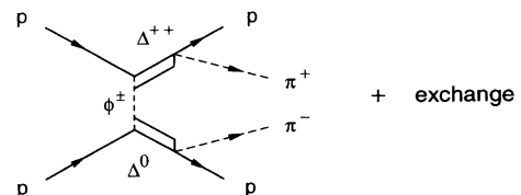
FIG. 7. Two-pion-production diagrams proceed via NN \rightarrow \Delta\Delta \rightarrow NN\pi\pi .
