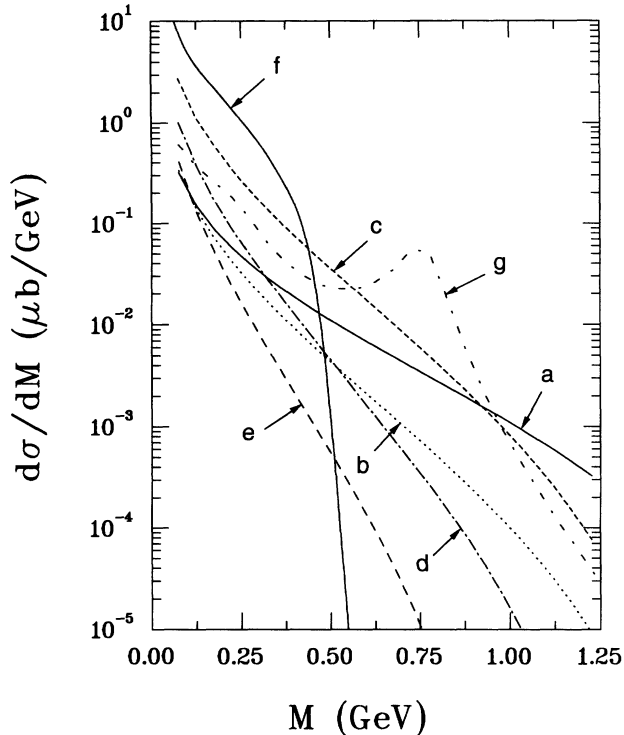
FIG. 11. Cross sections without any experimental acceptance included. Labels indicate the following mechanisms: (a) simple proton-proton bremsstrahlung in the solid line, (b)–(e) are pp\pi^0 in the dotted line, np\pi^+ in the short-dashed line, pp\pi^+\pi^- in the dot-dashed line, and np\pi^+\pi^+\pi^- final state bremsstrahlung in the long-dashed line; (f) is eta Dalitz decay and finally, radiative Delta decay is shown in curve (g).
