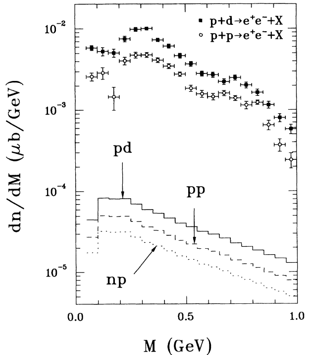
FIG. 4. Dilepton yield from simple pp and np bremsstrahlung as compared with DLS data from Ref. [1] for 4.9 GeV proton-proton (open circles) and proton-deuteron (solid squares) inclusive reactions. Our pp result is shown as the dashed histogram, np is shown as the dotted histogram, and an approximate pd = pp + np is shown as the solid histogram.
