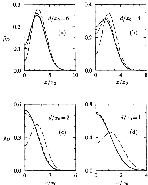
FIG. 1. The adimensional baryon density of the two-nucleon bound state for various values of the ratio d/x_0 of bound-state size to nucleon size. Full line, soliton model; dot-dashed line, quark model; dashed line, convolution of the single-nucleon density with the probability density for the relative position of the nucleon centers.
