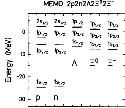
FIG. 9. Single-particle energy of a MEMO consisting of two of each baryon of the baryon octet except the \Sigma 's. The binding energy difference cancels the mass difference of the strong reaction channels so that the whole “nucleus” is metastable.
