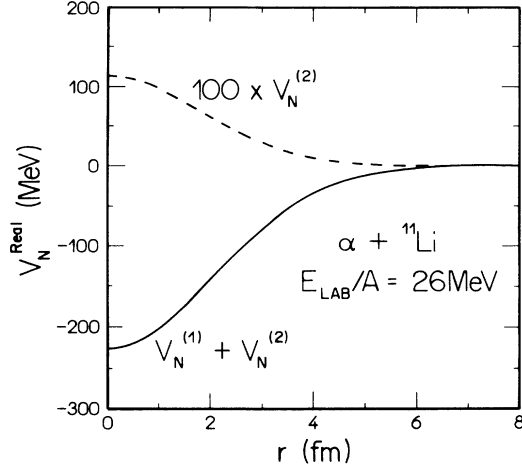
FIG. 3. Real part of the second-order correction for the \alpha + {}^{11}\text{Li} optical potential (dashed line). The solid line is the sum of the first- and second-order potentials [Eqs. (3.1) and (3.3)].
