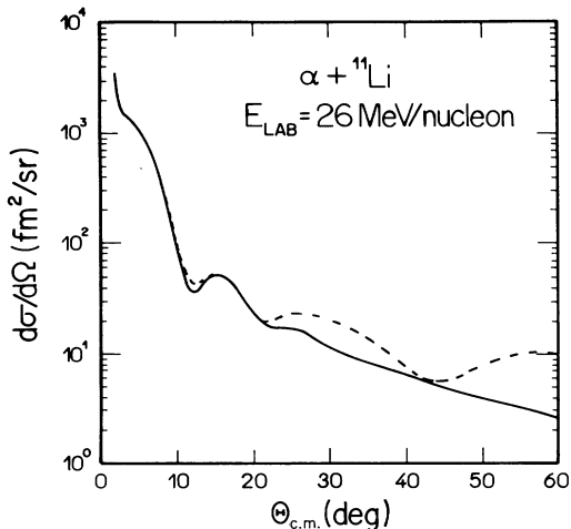
FIG. 6. Elastic cross section for the system \alpha + {}^{11}\text{Li} at 26 MeV/nucleon. The dashed line was calculated with the first-order optical potential. The solid line includes the contribution of the second-order potential.
