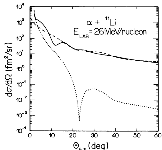
FIG. 9. Near- (dotted curve) and farside (dashed curve) contribution to the elastic scattering cross section (solid) for the system \alpha + {}^{11}\text{Li} at 26 MeV/nucleon.
