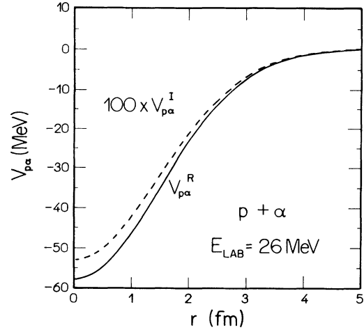
FIG. 1. Imaginary part (dashed curve) and real part (solid curve) of the optical potential for p + \alpha scattering.
