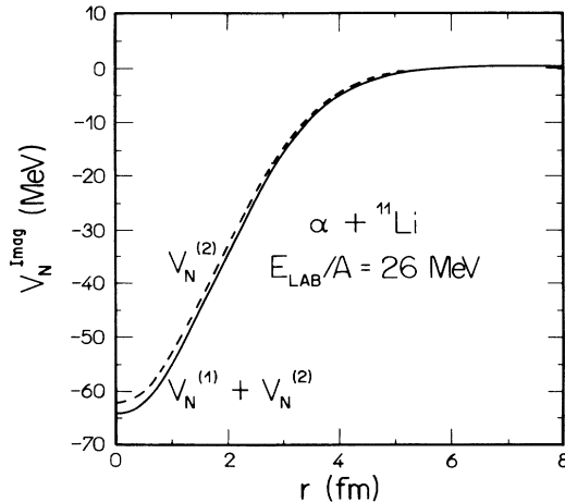
FIG. 4. Same as Fig. 3, but for the imaginary part of the potentials.
