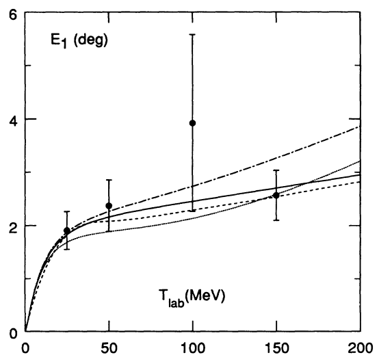
FIG. 1. Mixing parameter \varepsilon_1 in degrees versus T_{\text{lab}} in MeV. Black dots: single-energy result; solid curve: multi-energy result; dash-dotted curve: Nijmegen potential; dotted curve: Paris potential; dashed curve: Bonn potential.
