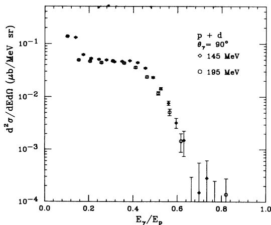
FIG. 3. Comparison of the energy spectra at 90^\circ in the laboratory for deuterium at 145 and 195 MeV vs a reduced variable E_\gamma/E_p , which is the measured photon energy divided by the incident proton energy.
