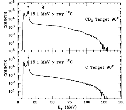
FIG. 1. Gamma ray energy spectra at 90^\circ in the laboratory for both the C (lower frame) and \text{CD}_2 (upper frame) targets at 145 MeV. The 15.1 MeV gamma ray transition in ^{12}\text{C} is clearly observed.
