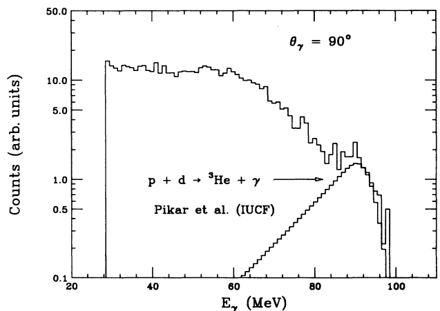
FIG. 2. Bremsstrahlung gamma ray spectrum for deuterium at 145 MeV; also shown is a comparison of the radiative capture peak p + d \rightarrow {}^3\text{He} + \gamma . The capture peak is generated by using the value for the radiative capture process measured by Pikar et al. [20] and a procedure described in the text.
