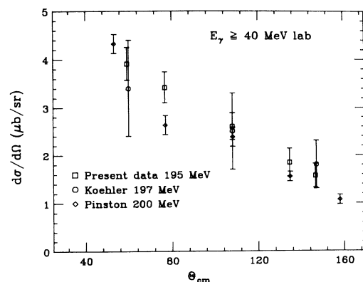
FIG. 5. Comparison of the measured angular distribution for pd\gamma at 195, 197 [16], and 200 MeV [17].
