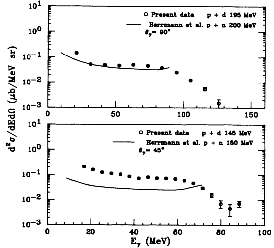
FIG. 6. Comparison of the measured pd\gamma energy spectra at 145 and 195 MeV in the nucleon-nucleon center-of-mass frame with the free pn\gamma calculation of Herrmann, Speth, and Nakayama at 150 and 200 MeV [21].
