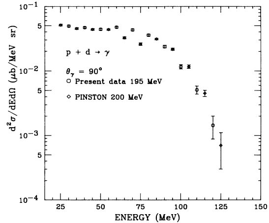
FIG. 4. Comparison of the gamma ray energy spectra for deuterium at 195 MeV to the data of Pinston et al. at 200 MeV [17]. Both energy spectra have been corrected for the radiative capture cross section.
