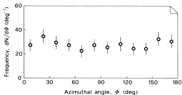
FIG. 1. Azimuthal angle distribution of ^{238}\text{U} fission fragments obtained from normal incidence of a polarized and monochromatic photon beam of 59.5-MeV maximum energy (photon beam energy of 52 MeV).
