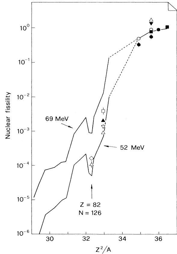
FIG. 2. Nuclear fissility plotted against parameter Z^2/A . Experimental results (points) obtained at 52-MeV photon mean energy are those as reported in Table I: (■), ^{237}\text{Np} and ^{238}\text{U} (Ref. [4]); (○) ^{235}\text{U} , ^{238}\text{U} , and ^{232}\text{Th} (Ref. [5]); (△) ^{238}\text{U} , ^{209}\text{Bi} , and ^{208}\text{Pb} (Ref. [6]); (▼), ^{238}\text{U} (Ref. [7]); (□) ^{209}\text{Bi} (Ref. [8]); (▽) ^{209}\text{Bi} (Ref. [9]); (▲) ^{209}\text{Bi} (D. Türck et al. , quoted in Ref. [9]); (◇) ^{208}\text{Pb} (Ref. [10]); (●) ^{235}\text{U} , ^{238}\text{U} , and ^{232}\text{Th} (this work). The broken lines connect fissility values estimated at 52- (this work) and 69-MeV (Ref. [1]) excitation energy. The dashed lines are used for regions of Z^2/A where the ratio a_f/a_n is not known from experiment (for details see text).
