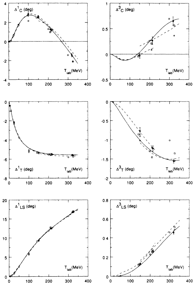
FIG. 2. Phase-shift combinations of {}^3P and {}^3F waves in degrees vs T_{lab} in MeV. Errors are shown for our SE results (bullets) only. Curves and symbols have the same meaning as in Fig. 1.
