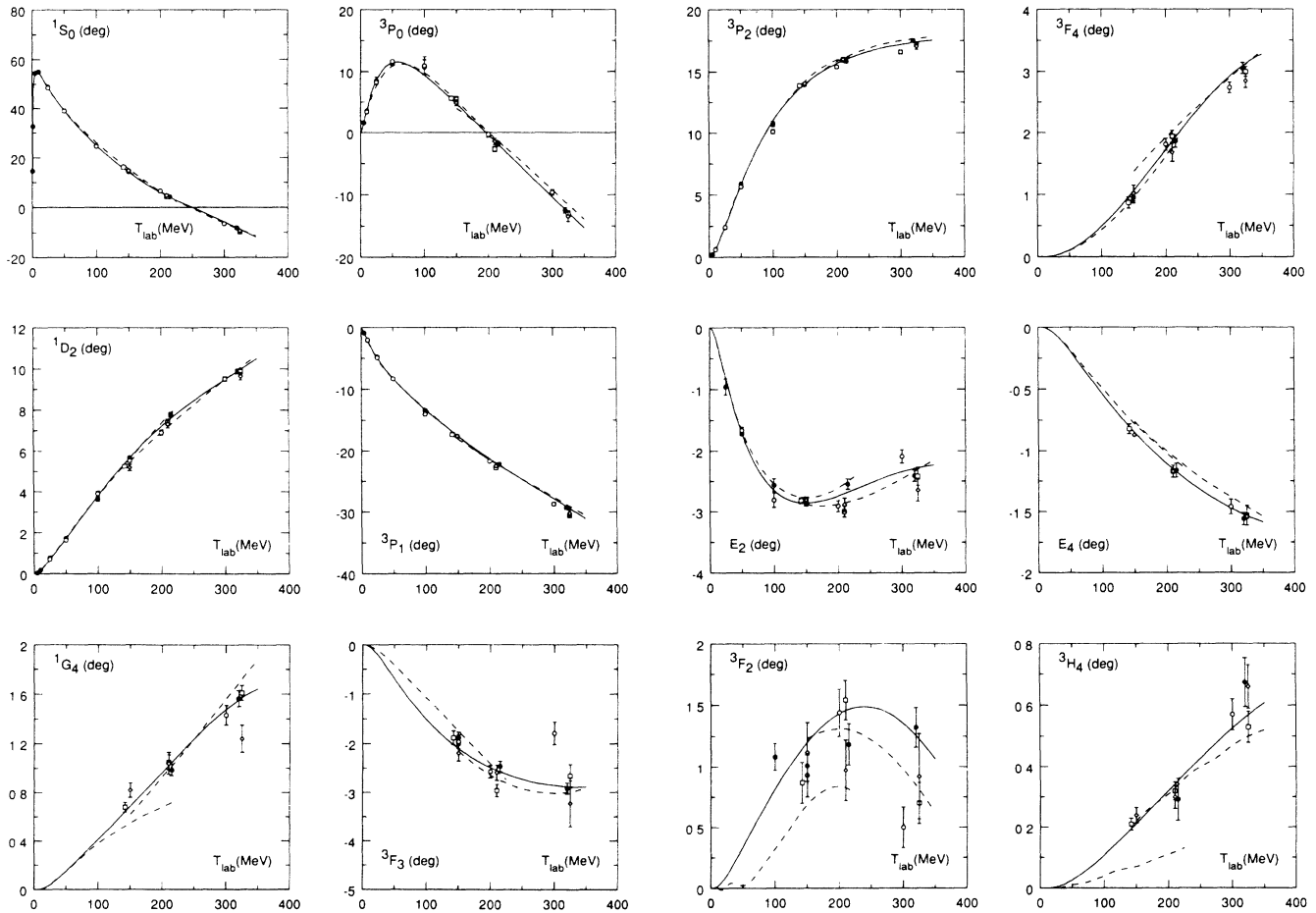
FIG. 1. Phase shifts in degrees vs T_{\text{lab}} in MeV. Errors are shown only if they are large enough to be plotted. Solid line: multienergy analysis; dashed line: Bystricky et al. (Ref. 6). ●: single-energy analysis; ○: Arndt et al. (Ref. 7); □: Dubois et al. (Ref. 18); ◇: Bugg et al. (Ref. 19).
