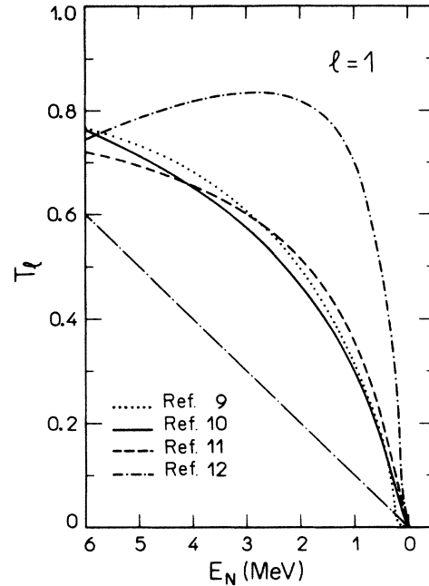
FIG. 3. The same as Fig. 2, but for l=1 .
