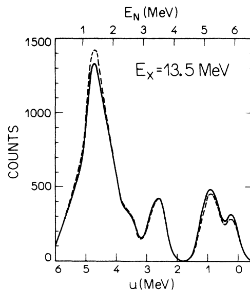
FIG. 8. Calculated statistical neutron decay spectra for the E0 GR in ^{208}\text{Pb} assuming a resolution of 500 keV. The continuous (dashed) line shows the result obtained with the optical potential of Ref. 9 (Ref. 11). The 141 experimental levels of ^{207}\text{Pb} that can be reached by the neutron decay are used (see the text).
