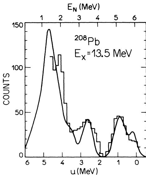
FIG. 10. The curve is the same calculation shown by the full line in Fig. 9. The histogram is the experimental neutron spectrum from Ref. 4. The calculated spectrum was normalized to fit the intensity of fast neutrons in the experimental spectrum.
