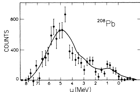
FIG. 12. The same experimental data as in Fig. 11 and the same statistical calculation but for an energy resolution of 2.4 MeV.
