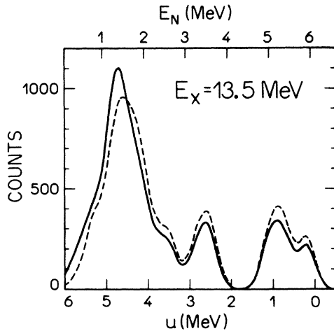
FIG. 9. Calculated statistical neutron decay spectra for the E_0 GR in ^{208}\text{Pb} , using the optical potential of Ref. 11. The dashed line shows the result obtained using 78 experimental levels of ^{207}\text{Pb} as in the calculation of Ref. 1, and the full line the result obtained using 63 additional levels from a recent compilation. Both spectra are normalized to the same number of neutrons.
