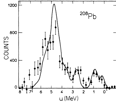
FIG. 11. Calculated neutron spectrum from an excitation energy of 14 MeV in ^{208}\text{Pb} and an energy resolution of 500 keV. The experimental points are from Ref. 6. The calculated spectrum is normalized to the total number of neutrons in the experimental spectrum.
