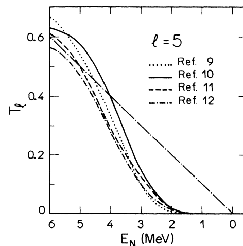
FIG. 7. The same as Fig. 2, but for l=5 .
