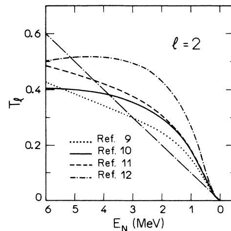
FIG. 4. The same as Fig. 2, but for l=2 .
