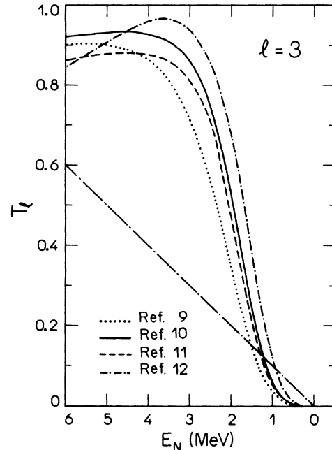
FIG. 5. The same as Fig. 2, but for l=3 .
