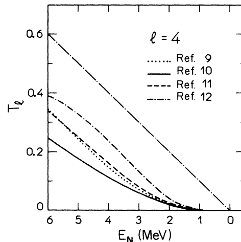
FIG. 6. The same as Fig. 2, but for l=4 .
