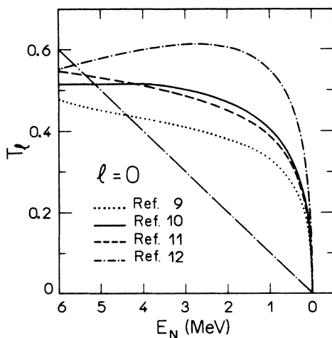
FIG. 2. Transmission coefficients for l=0 and different parametrizations of the optical potential. The straight line represents the assumption of a transmission coefficient independent of l and directly proportional to the neutron energy (see the text).
