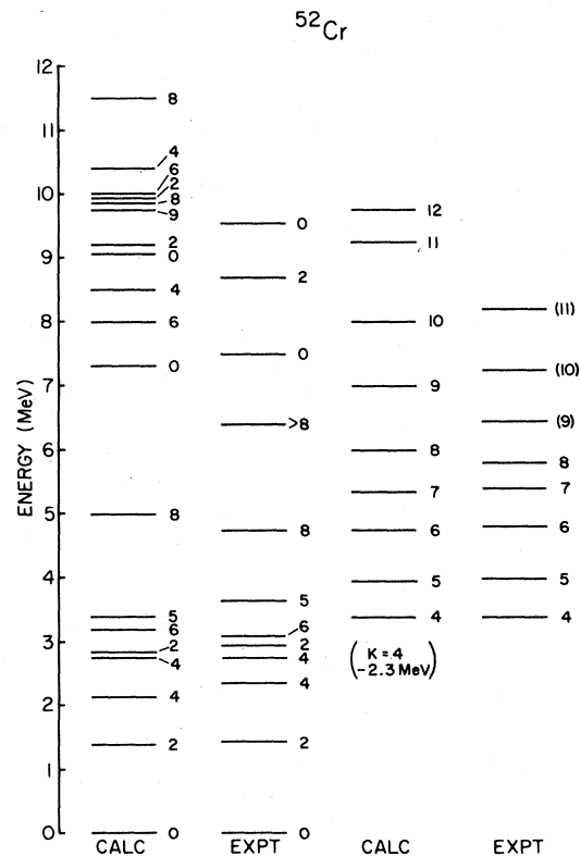
FIG. 4. The theoretical and experimental energy spectra of positive parity states in 52 Cr. The left hand part of the spectrum exhibits levels belonging to the ground state band with a predominant (0f_{7/2})^n component, whereas the right-hand part of the spectrum shows the collective band of states belonging to the deformed K^\pi=4^+ band.
