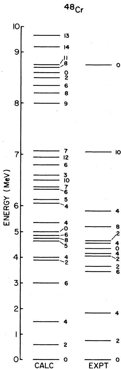
FIG. 1. Comparison of theoretical and experimental energy spectra for positive parity states in 48 Cr. The numbers on the right of the levels indicate J values.
