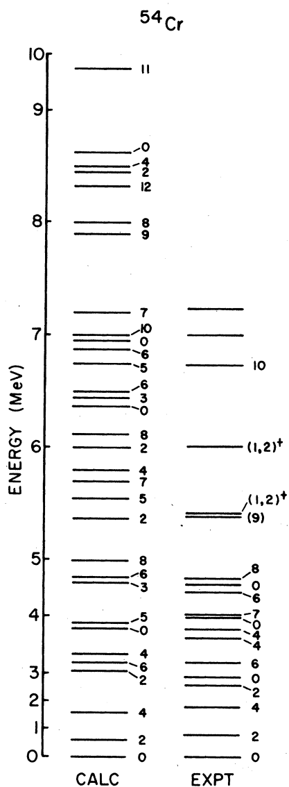
FIG. 5. The calculated and experimental energy spectra of positive parity states in ^{54}\text{Cr} . Other details are the same as in Fig. 1.
