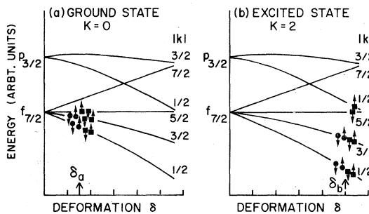
FIG. 2. The schematic Nilsson diagram for the ground and excited intrinsic states of ^{50}\text{Cr} with prolate deformation. The excited intrinsic state is obtained by 1p-1h elementary neutron excitation. The ground and the excited intrinsic states correspond to the filling of the deformed orbitals at different deformations \delta_a and \delta_b , respectively.
