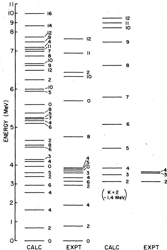
FIG. 3. The theoretical and experimental energy spectra of positive parity states in ^{50}\text{Cr} . The right hand part of the spectrum shows the collective band of states projected from K^\pi=2^+ deformed band. The numbers on the right of the levels indicate J values.
