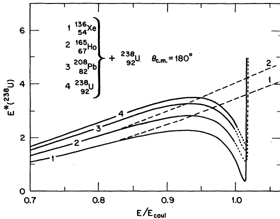
FIG. 2. Mean Coulomb excitation energy of ^{238}\text{U} for various projectiles and bombarding energies. The dashed curves have been calculated for a pure Coulomb potential, whereas the solid lines include destructive interference with the strong interaction (folded Yukawa potential).
