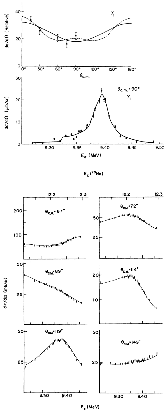
FIG. 6. The E_\alpha = 9.38 MeV resonance ( E_x = 12.24 MeV). Same format as Fig. 2. The \gamma_1 angular distribution indicates either a dipole (solid line, CL=0.35) or quadrupole (dashed line, CL=0.4) transition. The \gamma_1 excitation function fit (CL=0.3) is characteristic of our nonthick target yields. The solid line representing the global phase shift fit was omitted from the ES excitation functions in the region of the RC resonance to highlight the small deviations.
