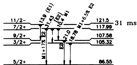
FIG. 4. Detail of decay of 118- and 121-keV levels.
