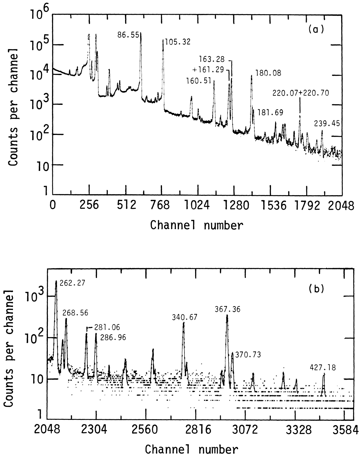
FIG. 1. \gamma -ray spectrum of mass separated ^{155}\text{Tb} measured with a high-resolution Ge(Li) spectrometer: (a) 0 to 250 keV and (b) 250 to 430 keV.
