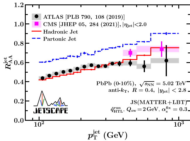
FIG. 20. Comparison of partonic jet R_{AA} with hadronic jet R_{AA} for two different parametrizations of \hat{q} . Jets are reconstructed with cone R = 0.4 at |y_{\text{jet}}| < 2.8 . The black circles are ATLAS data [114] and the dark red squares are CMS data for |\eta_{\text{jet}}| < 2.0 [120]. Top panel: Results for the formulation with virtuality dependence (Type 3). Bottom panel: Results for the \hat{q} formulation of the HTL with the running coupling (Type 2).
