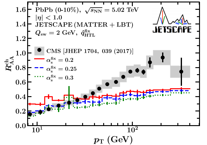
FIG. 16. Same as Fig. 6. For the \hat{q} formulation, the HTL with the fixed coupling (Type 1) is employed. The solid red, dashed blue, and dotted green lines show results with \alpha_s^{\text{fix}} = 0.2, 0.25, and 0.3 , respectively. Here we set Q_{\text{sw}} = 2 GeV.
