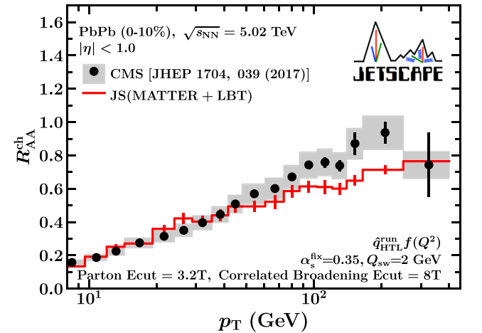
FIG. 23. Same as Fig. 6, but theoretical curves shows the results when partons with energy E \leq E_{\text{cut}} = 8T undergo nonperturbative energy loss modeled using correlated broadening. For the functional form of \hat{q} , the virtuality dependent formulation (Type 3) is employed. The solid red lines show the results with hadronization, and the dashed green line in the top panel shows the result for partonic jets.
