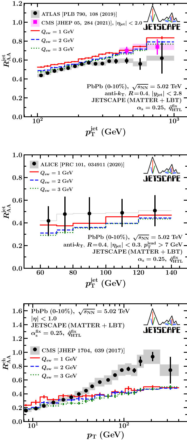
FIG. 17. Same as Fig. 6. For the \hat{q} formulation, the HTL with the fixed coupling (Type 1) is employed. The solid red, dashed blue, and dotted green lines show results with Q_{sw} = 1, 2, and 3 GeV, respectively. Here we set \alpha_s^{\text{fix}} = 0.25 .
