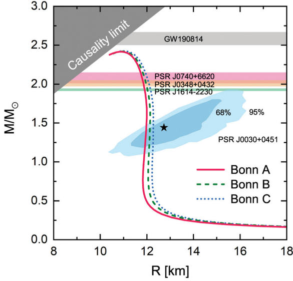
FIG. 3. The mass-radius relations of the neutron star obtained from the EOS by RBHF theory in the full Dirac space with the potentials Bonn A, B, and C. Astrophysical constraints from massive neutron star observations taken from Refs. [61–65] are shown as horizontal shaded areas. The dark and light blue regions indicate the 68% and 95% confidence intervals constrained by the NICER analysis of PSR J0030+0451 [57]. The recently inferred mass of the secondary compact object of GW190814 [66] is also shown. The gray region is excluded by causality that R > 2.9 GM/c^2 . See the text for details.
