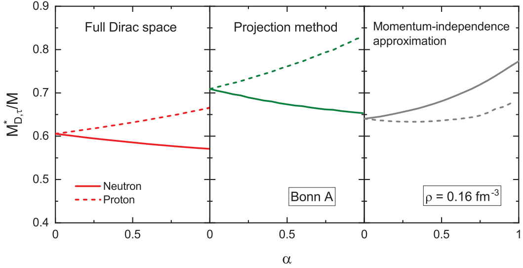
FIG. 1. Effective Dirac mass for the neutron (solid lines) and the proton (dashed lines) as functions of the asymmetry parameter \alpha at \rho = 0.16 \text{ fm}^{-3} calculated by the RBHF theory in the full Dirac space (left), in comparison with the results obtained by RBHF calculations with PESs only using the projection method [31] (middle) and the momentum-independence approximation [30] (right). The Bonn-A potential [49] is used.
