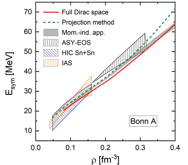
FIG. 2. The symmetry energy E_{\text{sym}} as a function of the density \rho calculated by the RBHF theory in the full Dirac space (red solid line), in comparison with the results obtained by the RBHF calculation with the projection method (olive dashed line) and the momentum-independence approximation (Mom.-ind. app., gray band). The constraints from the HIC [51], the IAS [52], and the ASY-EOS experiments [53] are depicted with blue, yellow, and gray shadows, respectively.
